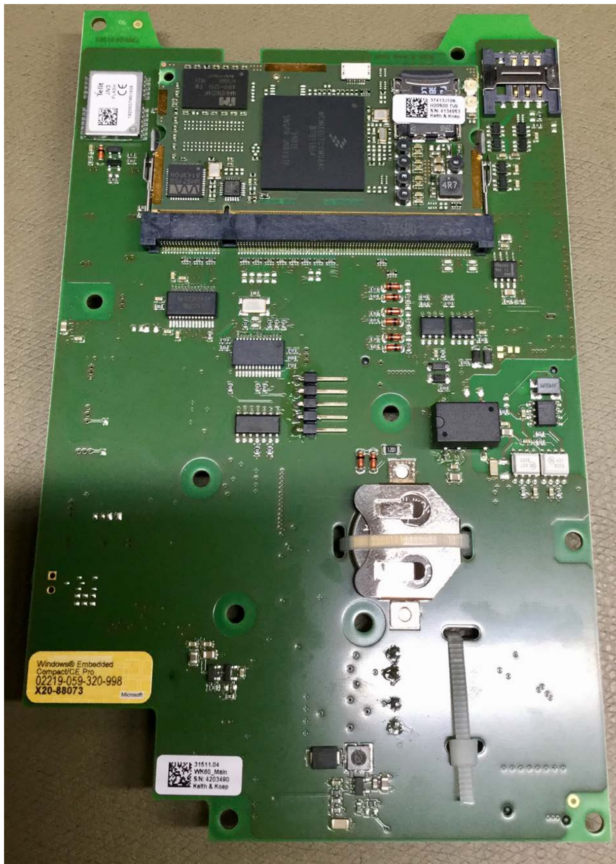
WK60_main_v1r4l1_top
