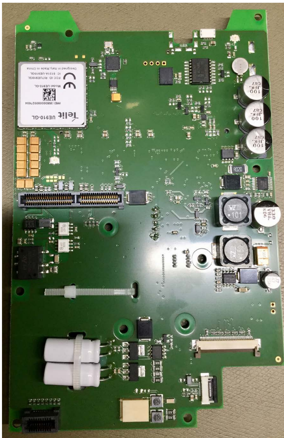
WK60_main_v1r4l1_bottom
