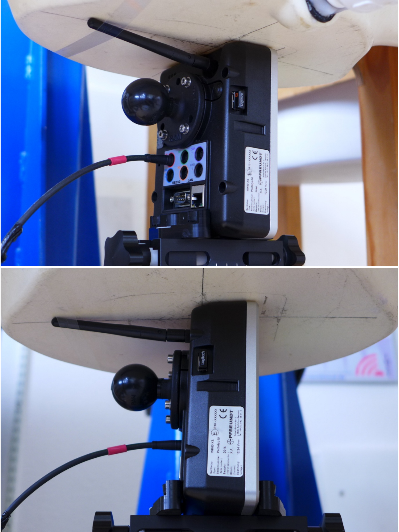
Fig. 9: Extremity exposure condition, top side of WK60-XS towards the phantom, 0 mm distance, antenna rotated forward.
