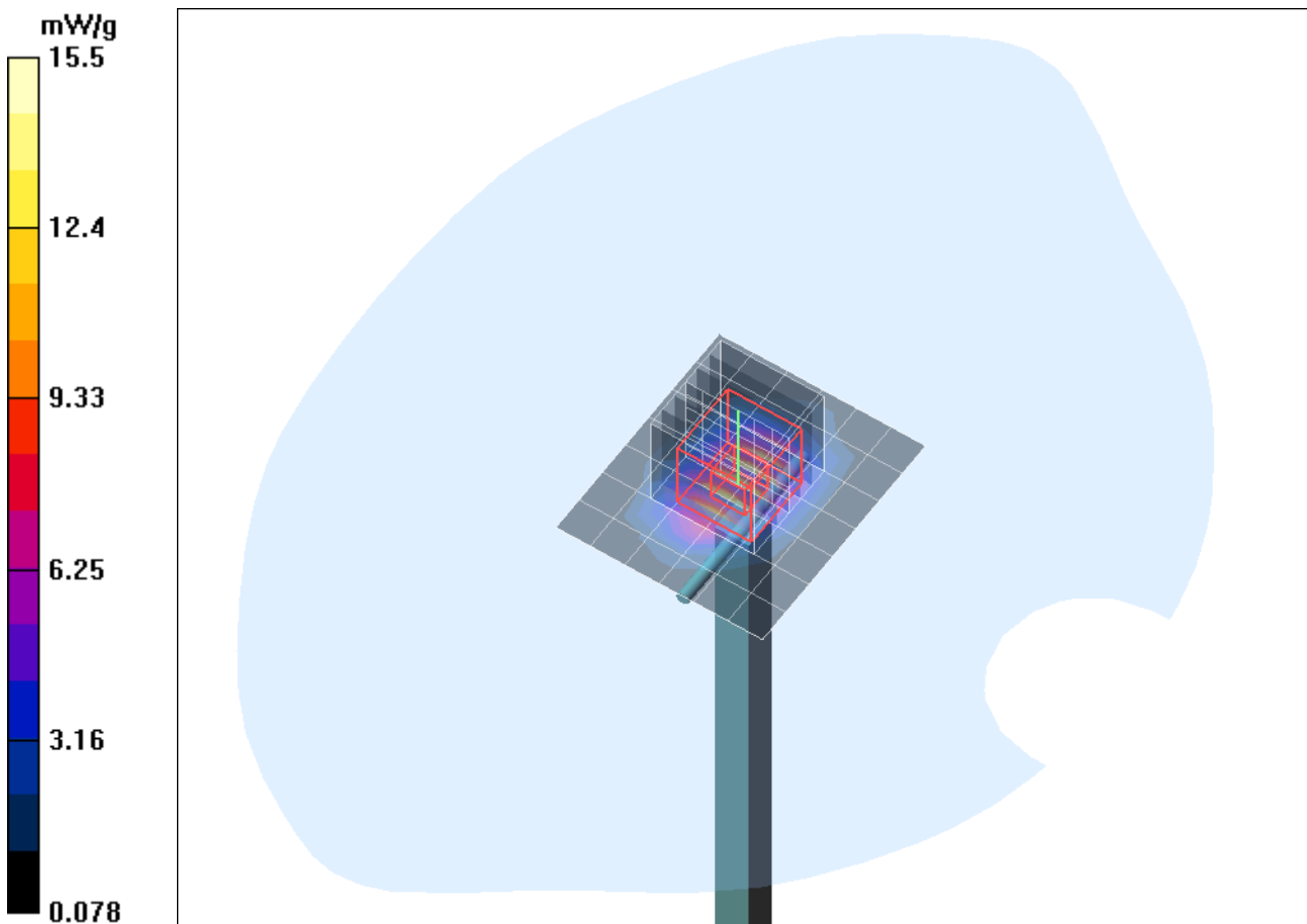
Fig. 4: System Check for 2450 MHz Body (July 6, 2016), coarse grid.
