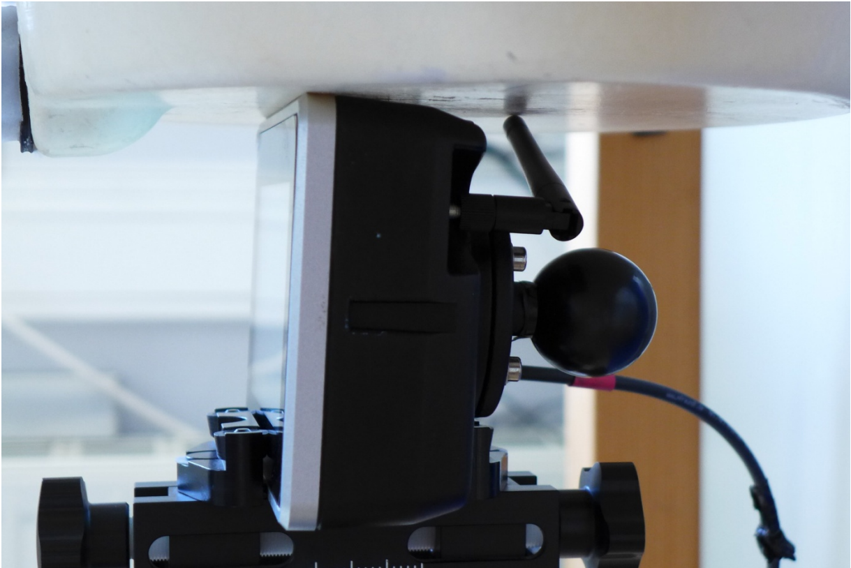
Fig. 12: Extremity exposure condition, left side of WK60-XS towards the phantom, 0 mm distance, antenna rotated down.
