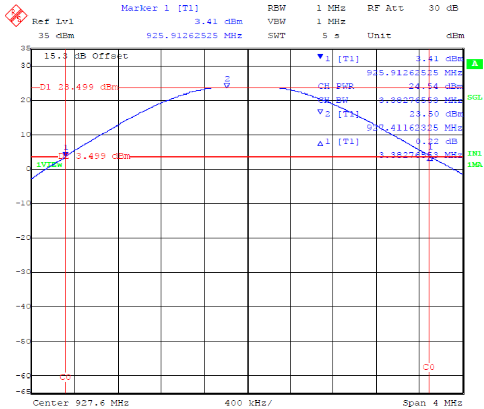
10kbps Channel 63
