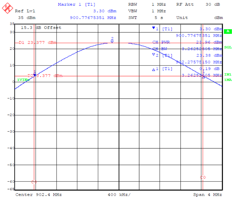
200kbps Channel 0
