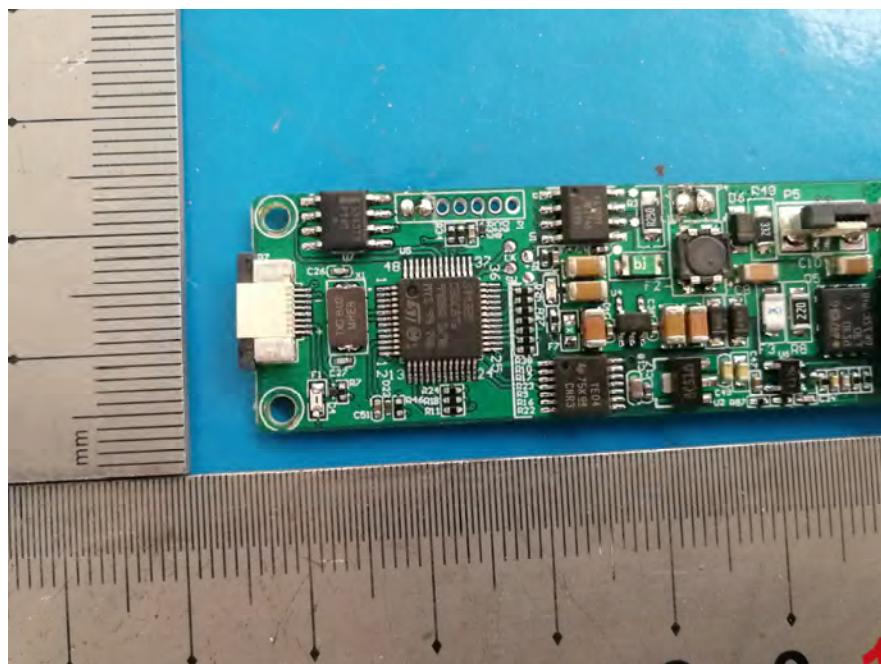
EUT – PCB-5 IC Chip View
