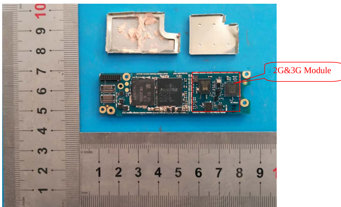
EUT – PCB-4 Bottom Shielding off View
