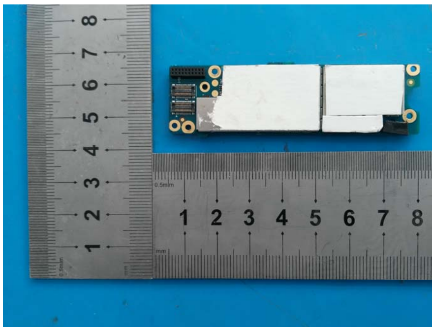
EUT – PCB-4 Bottom Shielding off View
