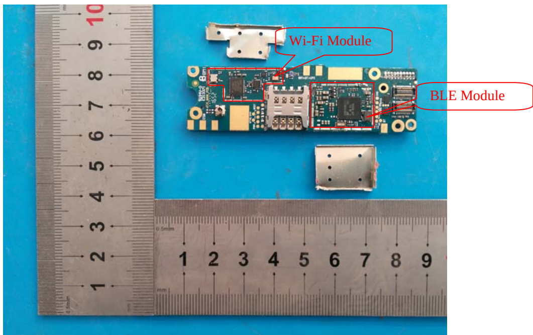
EUT – PCB-4 Top Shielding off View
