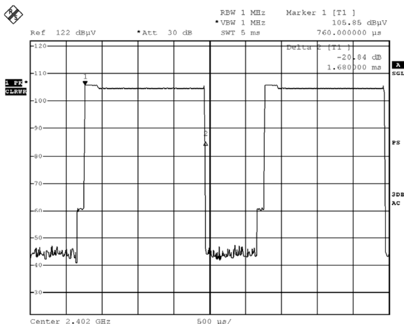
Fig. D [Pulse duration of Lowest Channel]
