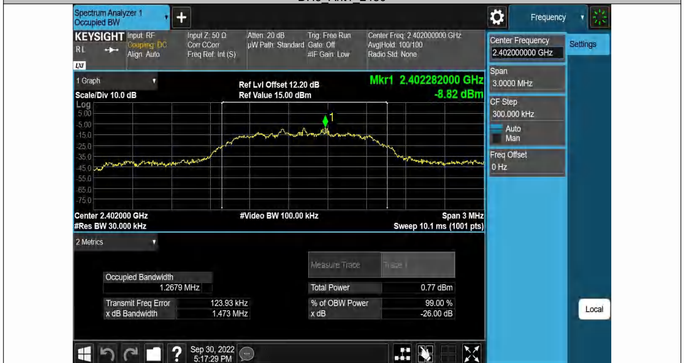
2DH5_Ant1_2402
