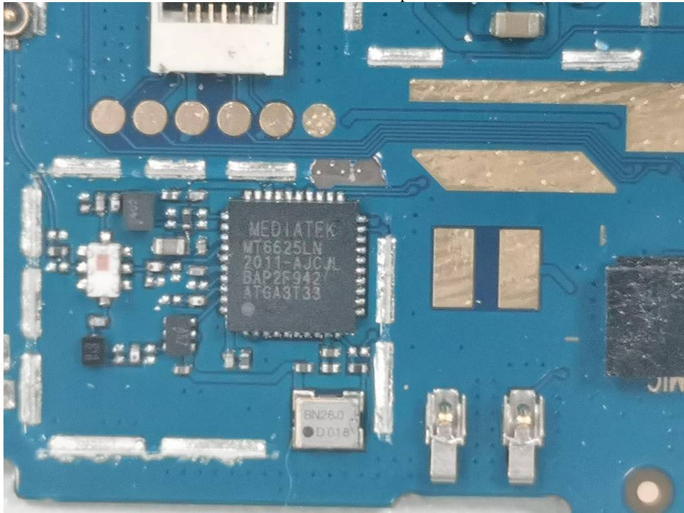
BT&WIFI Chip
