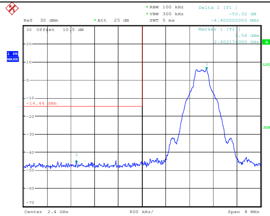
Band Edge, Single Channel
