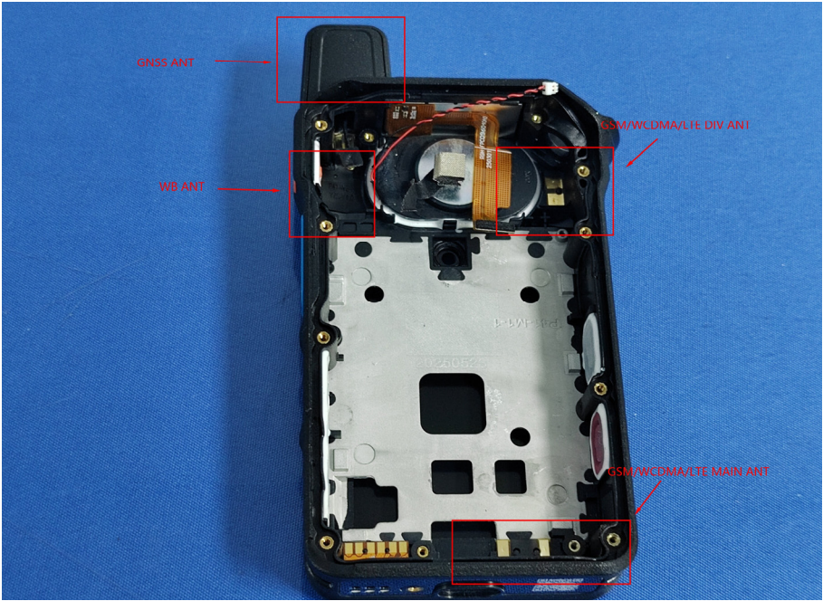
Antenna layout diagram
