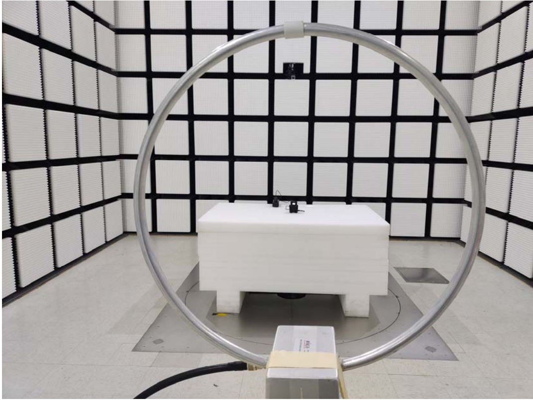
9kHz~30MHz _ Radiated Emission View - Perpendicular_ Charger
