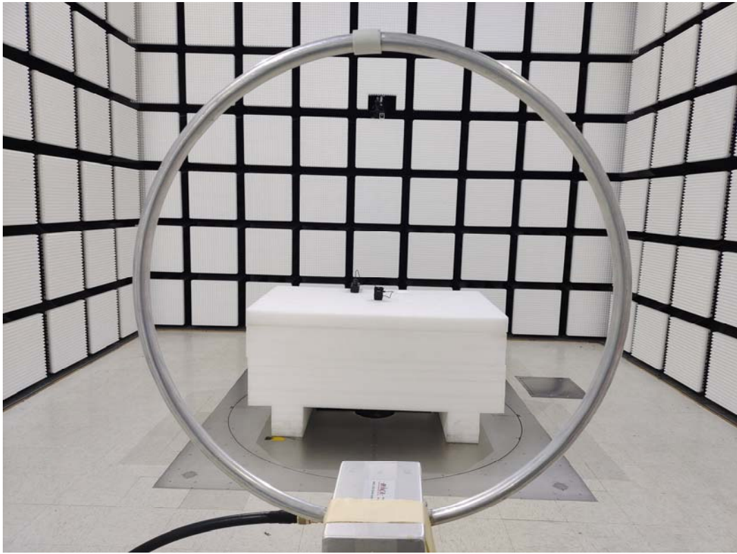
9kHz~30MHz _ Radiated Emission View - Perpendicular_ Adapter
