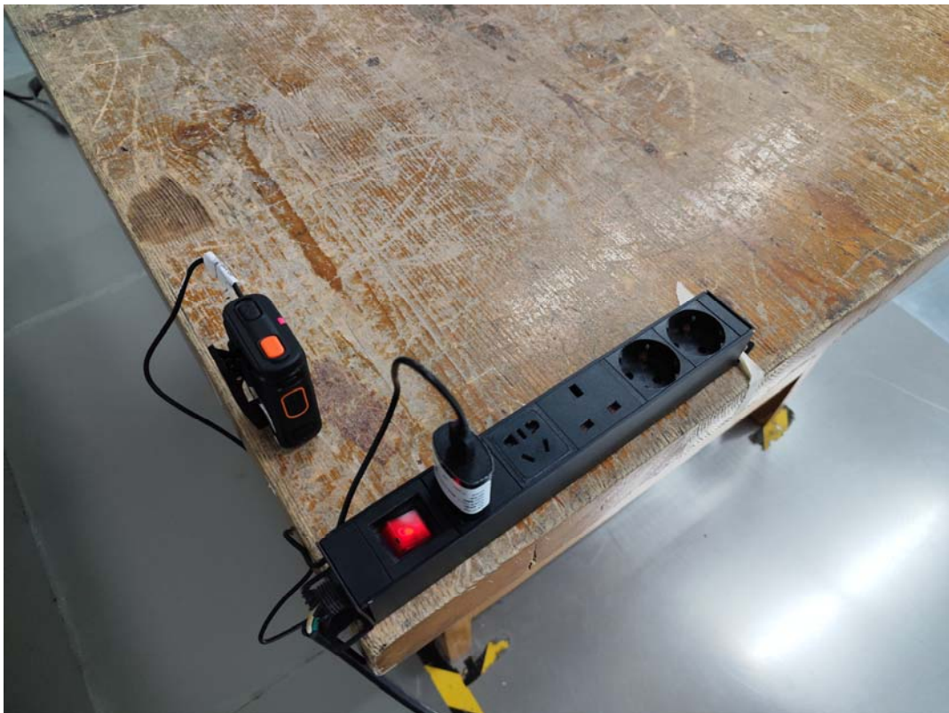
Conducted Emissions Side View_ Adapter
