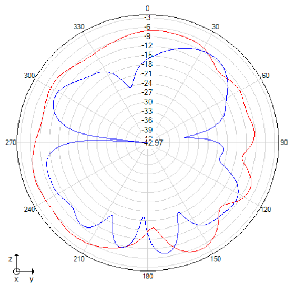
Phi=90 freq=2480MHz
