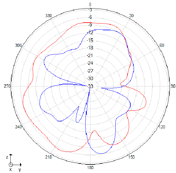
\Phi=90 freq=2300MHz
