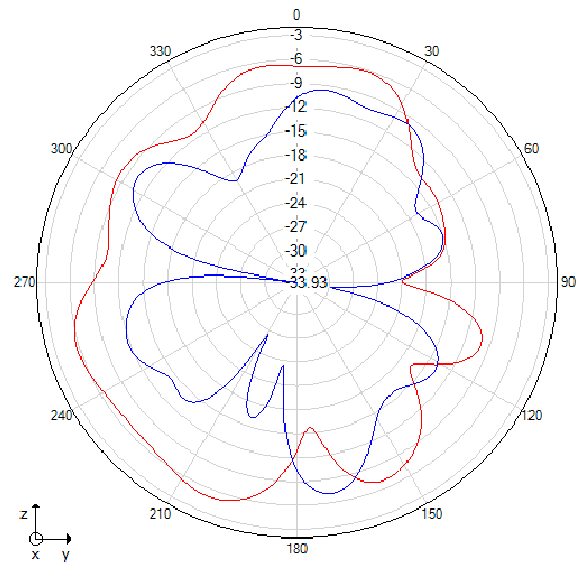
\Phi=90 freq=2320MHz
