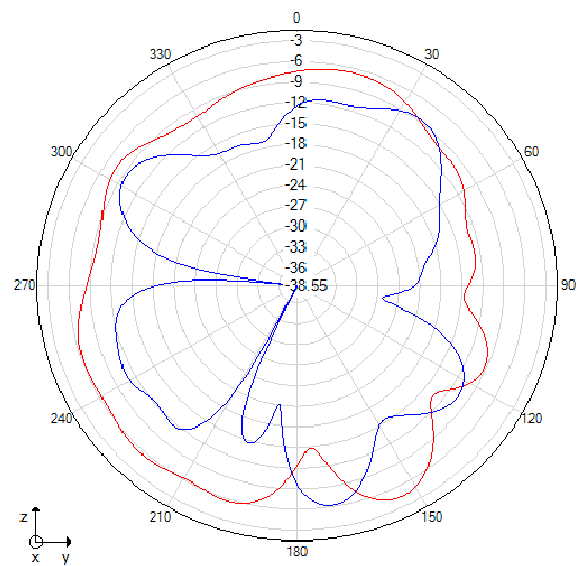
Phi=90 freq=2400MHz
