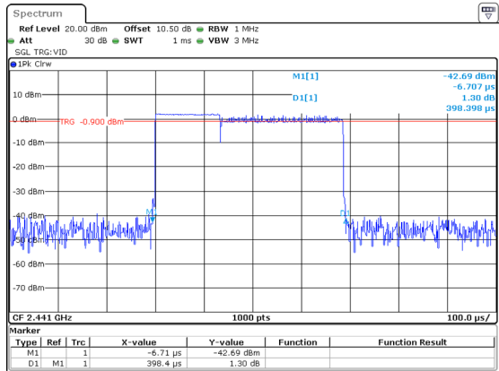
3DH1_Hopping 0.398ms
