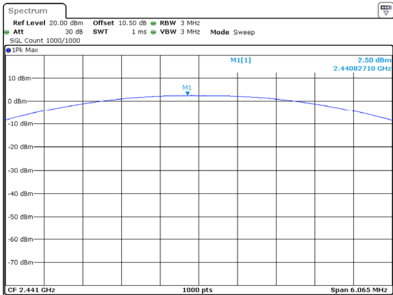
2DH1_Middle 2.50dBm
