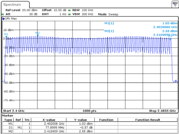
DH1_Hopping 79
