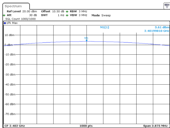
DH1_Low 3.61dBm
