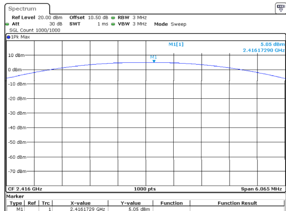
2DH1_Additional 5.05dBm
