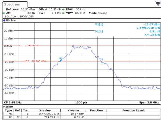
DH1_High 0.775MHz
