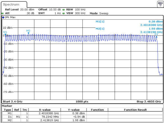
3DH1_Hopping 79
