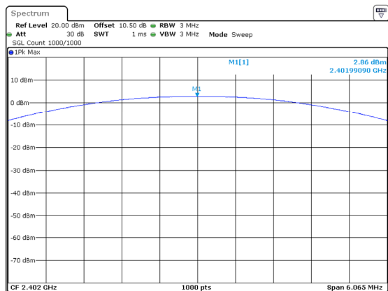
2DH1_Low 2.86dBm
