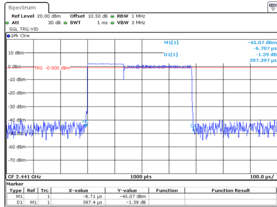
2DH1_Hopping 0.397ms
