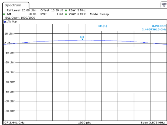
DH1_Middle 3.20dBm
