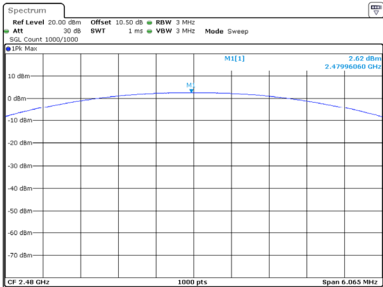
2DH1_High 2.62dBm
