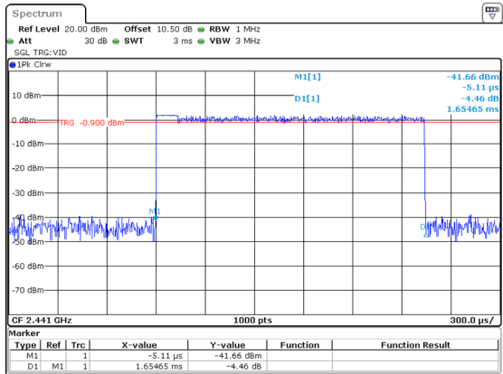
3DH3_Hopping 1.655ms
