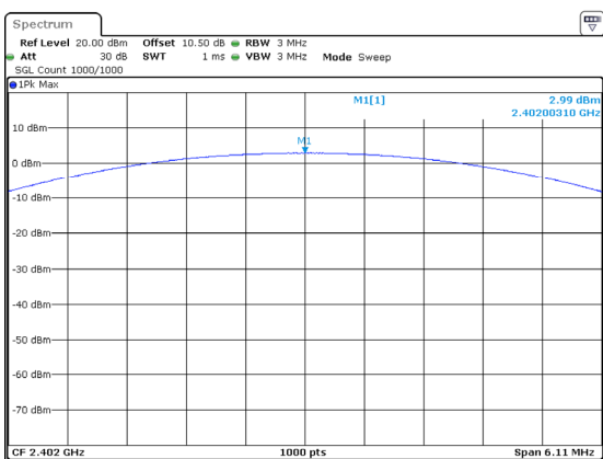
3DH1_Low 2.99dBm
