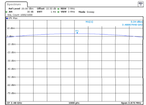
DH1_High 3.34dBm
