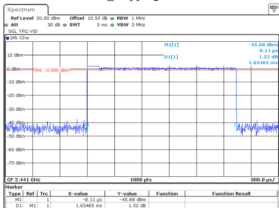
2DH3_Hopping 1.655ms
