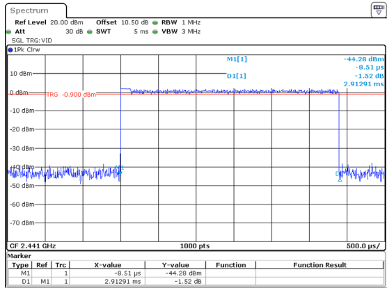
3DH5_Hopping 2.913ms
