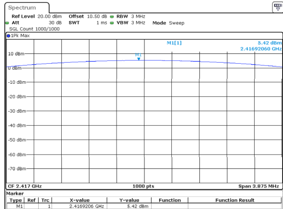
DH1_Additional 5.42dBm
