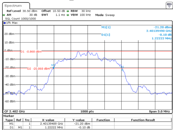
3DH1_Low 1.222MHz
