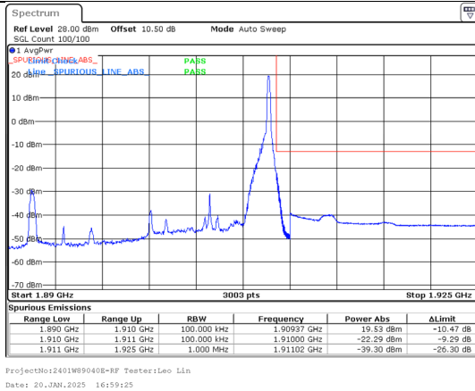
Band 2 10MHz/1905.0/High QPSK 1@49
