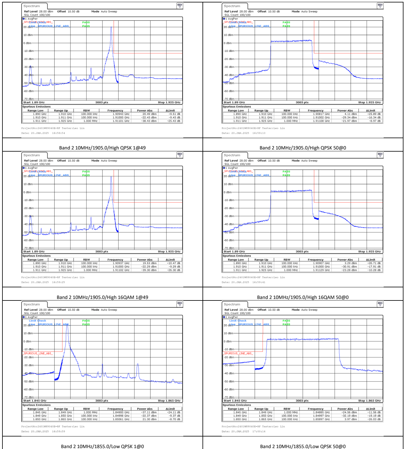
Band 2 10MHz/1855.0/Low QPSK 1@0
