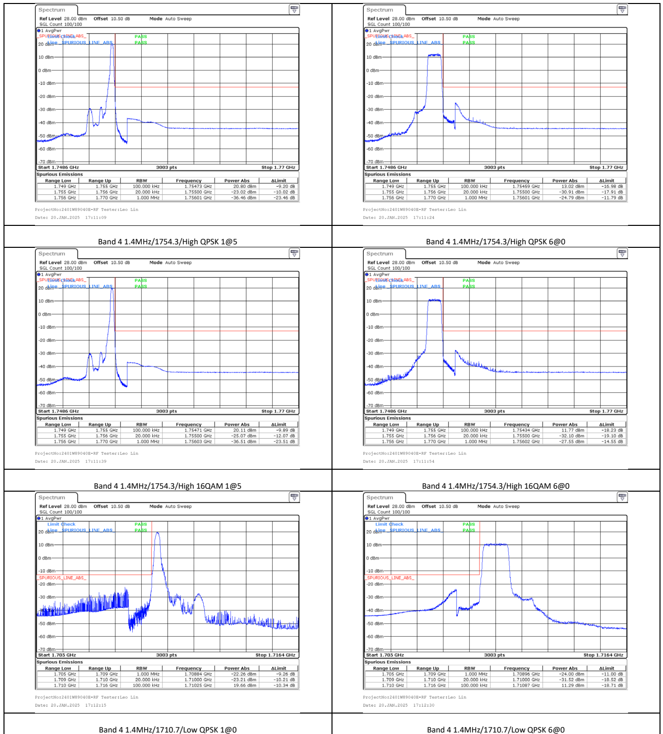
Band 4 1.4MHz/1710.7/Low QPSK 1@0
