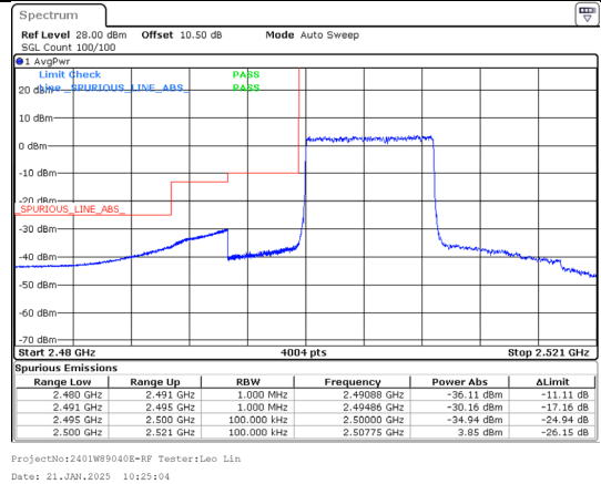
Band 7 10MHz/2505.0/Low 16QAM 50@0
