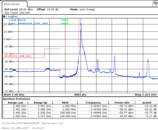
Band 7 10MHz/2505.0/Low 16QAM 1@0
