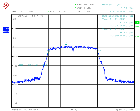
802.11g_2442MHz
