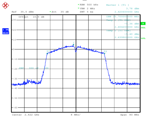
802.11n40_2422MHz
