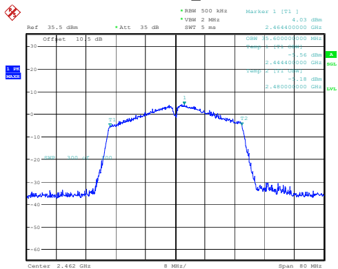
802.11n40_2462MHz
