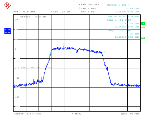
802.11g_2472MHz
