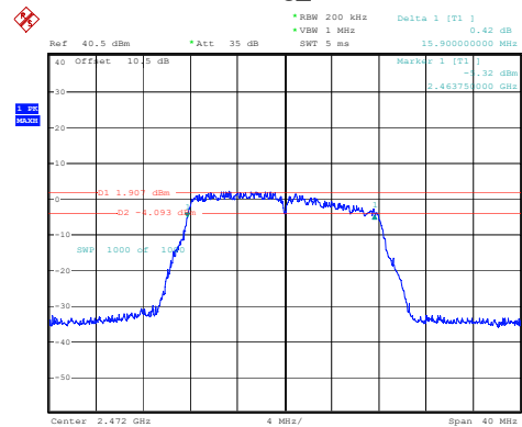
802.11g_2472MHz
