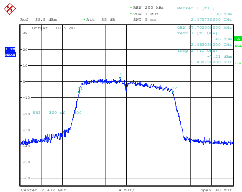
802.11n20_2472MHz
