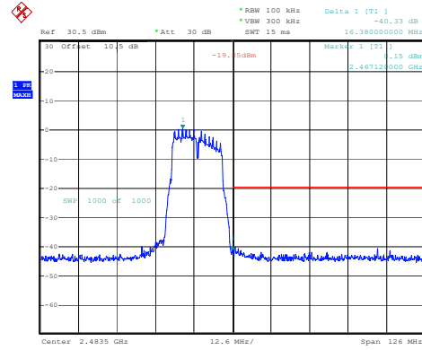
802.11g_2472MHz
