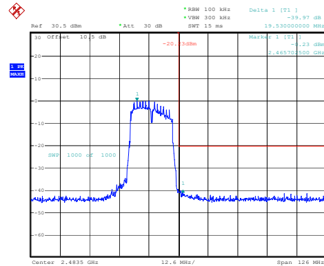
802.11n20_2472MHz
