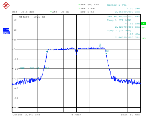
802.11n40_2442MHz
