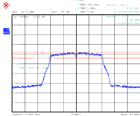
802.11g_2442MHz
