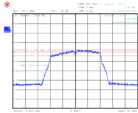
802.11g_2412MHz
