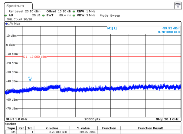
1.4MHz_Low_QPSK_6@0(1GHz~20.1GHz)
