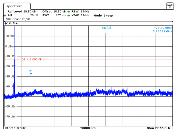
5MHz_Middle_QPSK_1@0(1GHz~27.55GHz)
