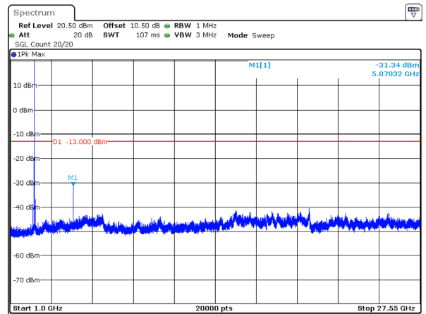
5MHz_Low_QPSK_1@0(1GHz~27.55GHz)
