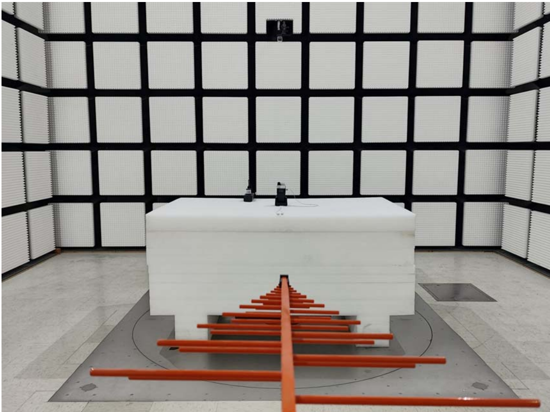
Radiated Emission Below 30M-1GHz View With Charging Base
