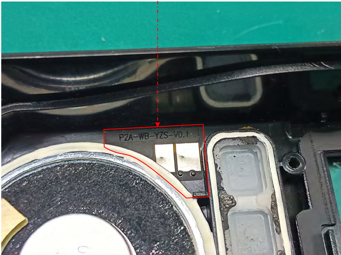
BT/Wi-Fi ANT
