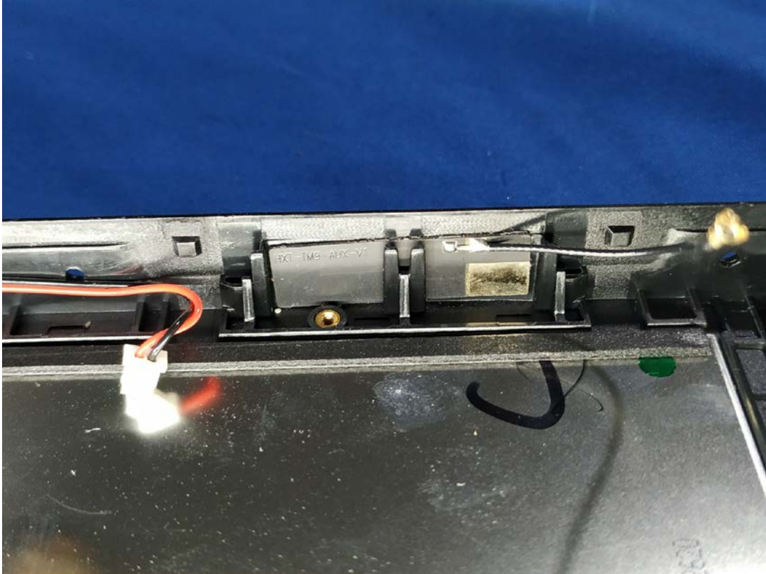
Aux Antenna
