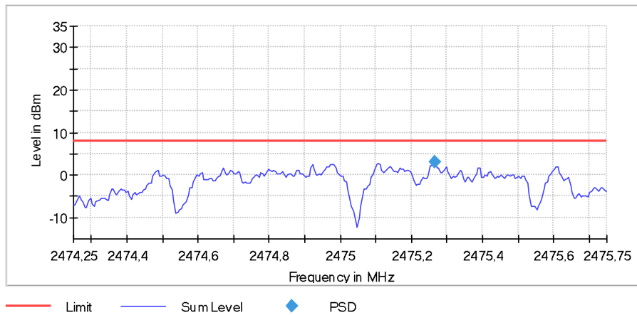
Channel 25 (2475 MHz)
