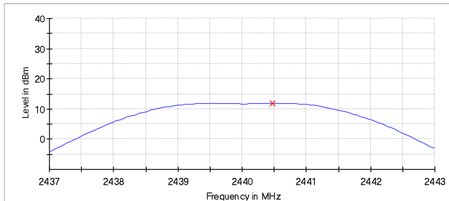
Channel 18 (2440 MHz)
