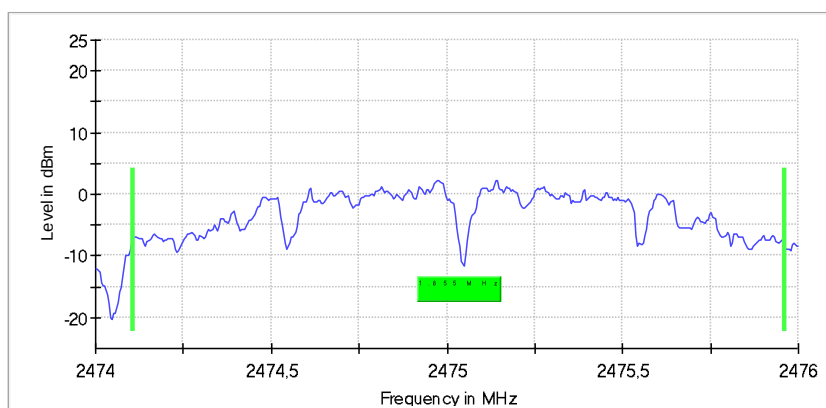
Channel 25 (2475 MHz)
