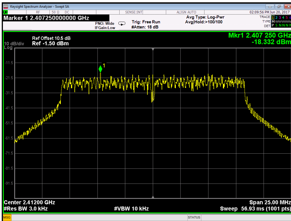
802.11n20 - Channel 1
