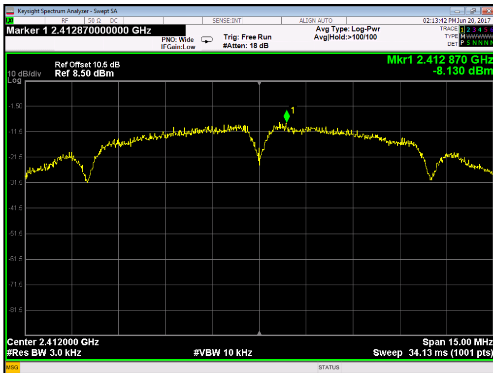
802.11b - Channel 1
