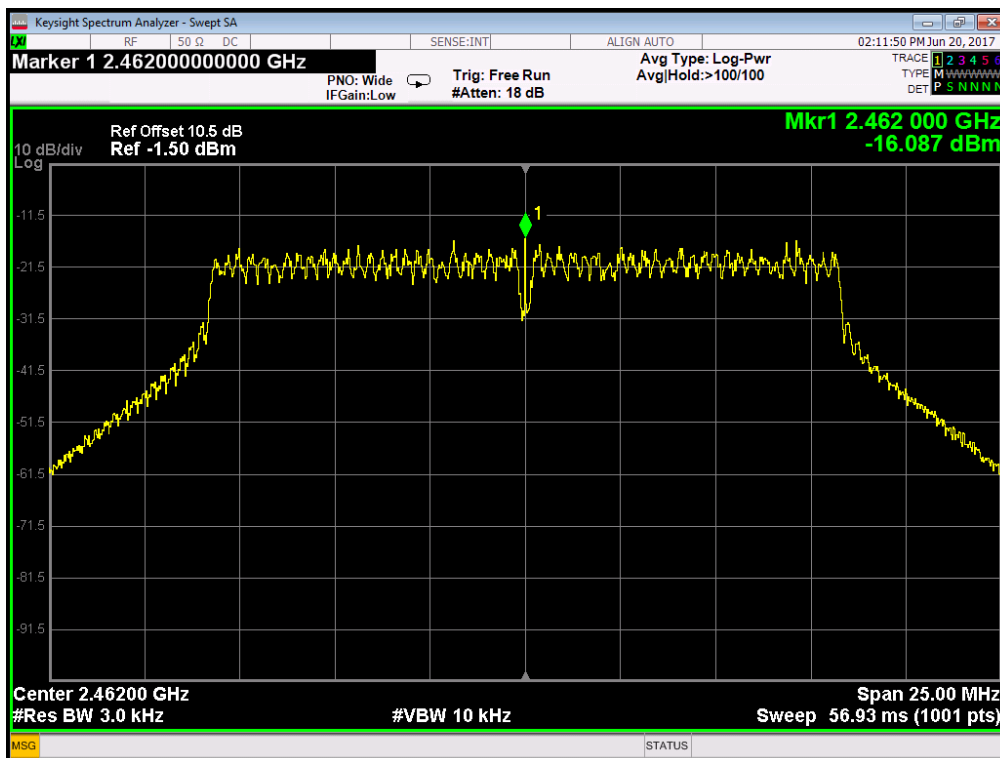
802.11g - Channel 11
