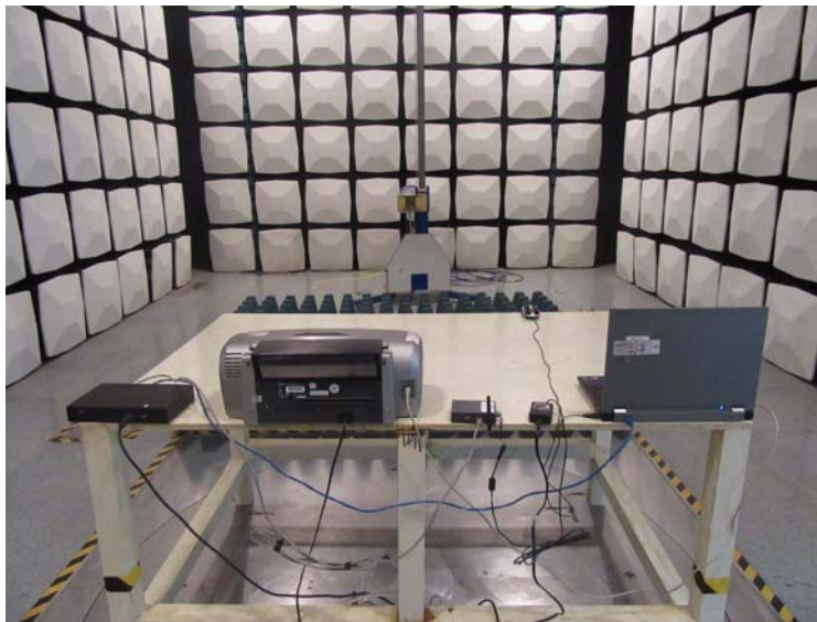
Radiated Emission Test Setup Rear View (Above 1 GHz)
