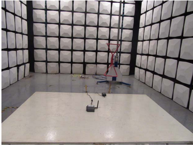
Radiated Emission Test Setup View (Below 1 GHz)
