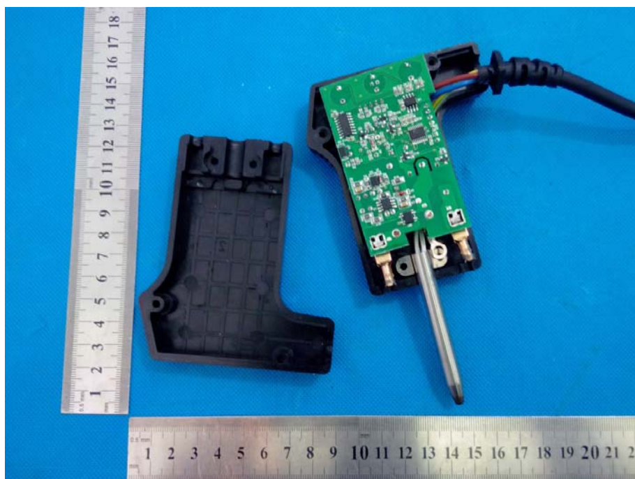
Temperature Controller 2#
