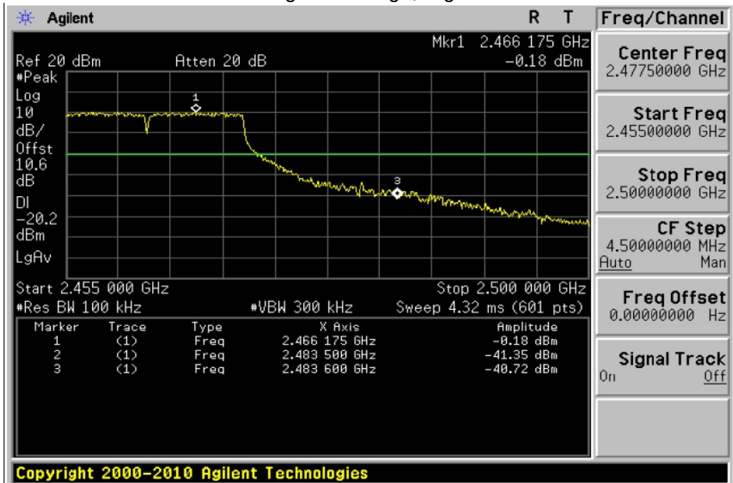
802.11g: Band Edge, Right Side
