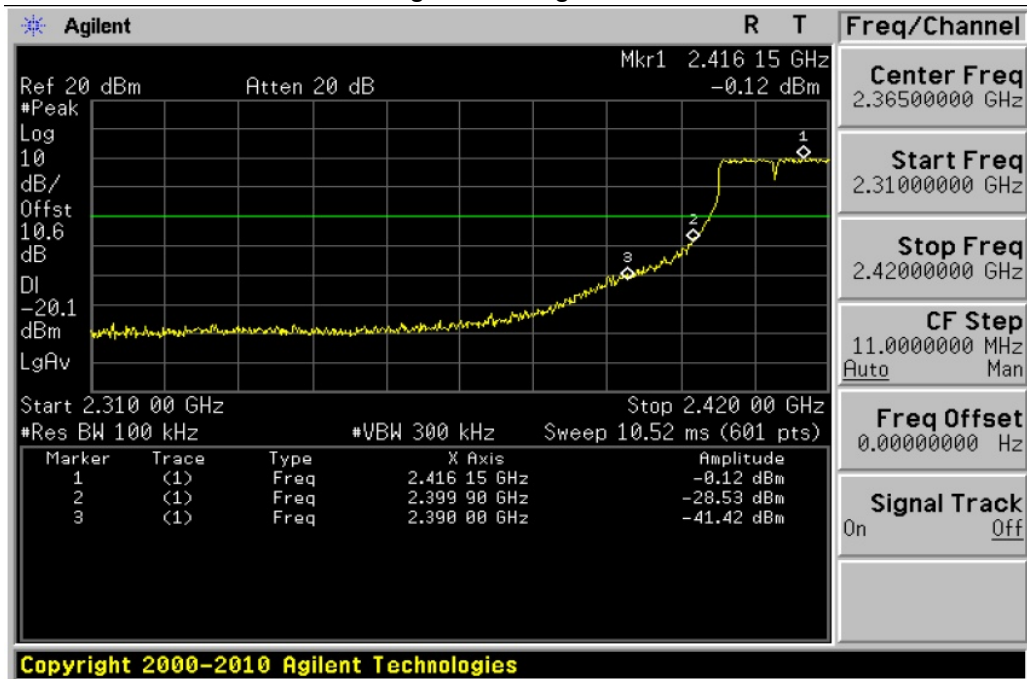
802.11g: Band Edge, Left Side
