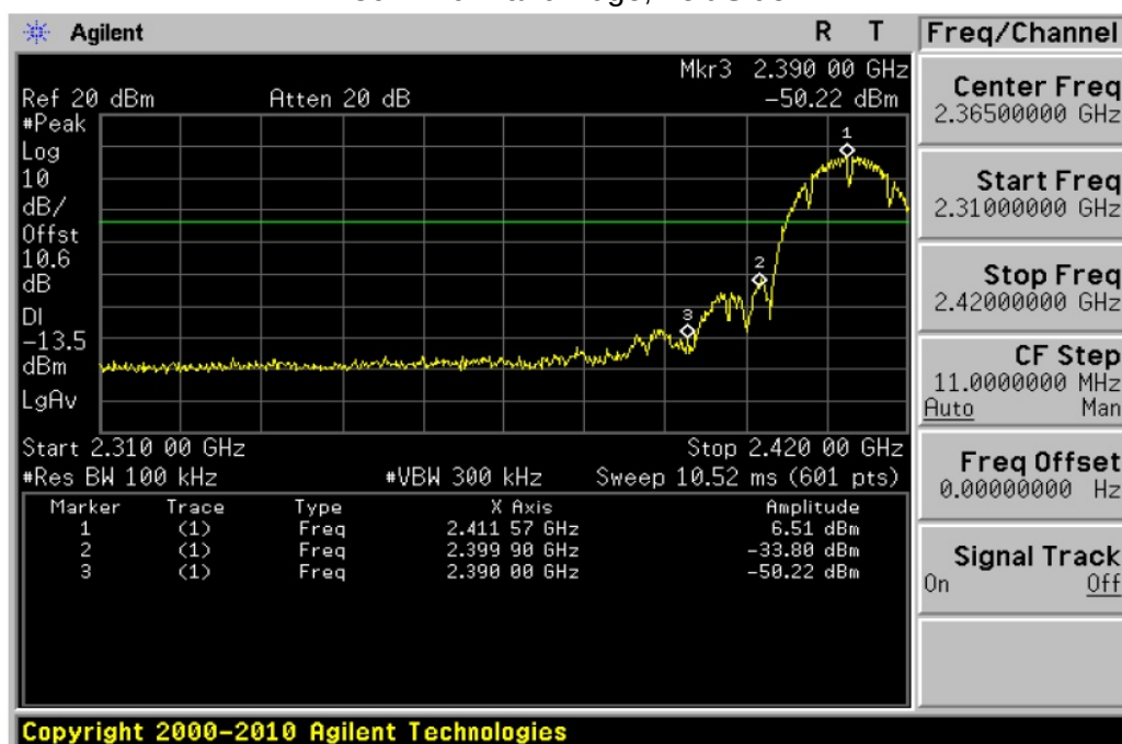
802.11b: Band Edge, Left Side
