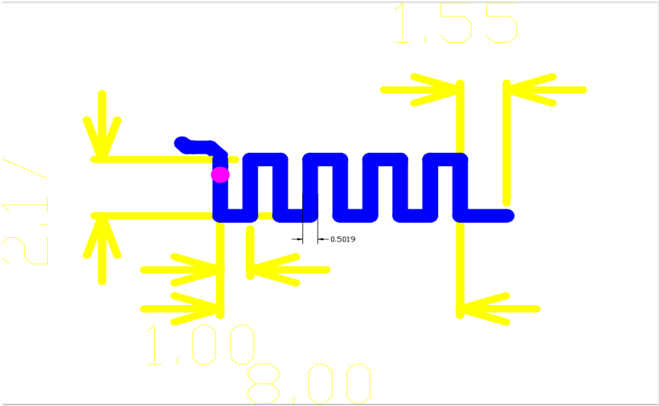
Antenna Photo & Length (mm)
