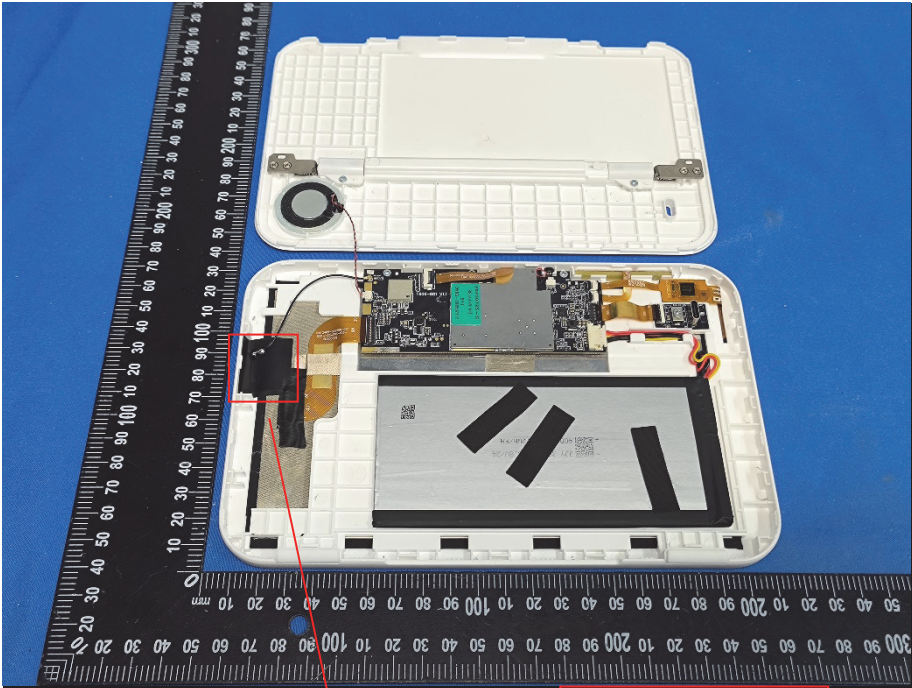
WIFI/Bluetooth Ant
