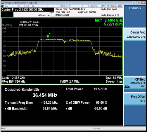
11N40SISO-Ant1-2452
