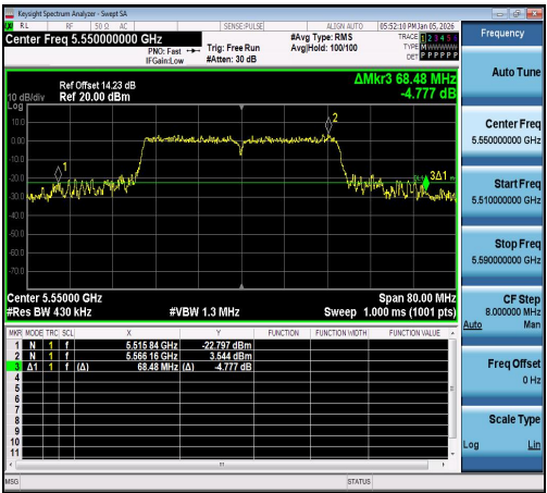
11N40SISO-Ant1-5550
