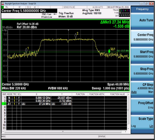
11AC20SISO-Ant1-5580
