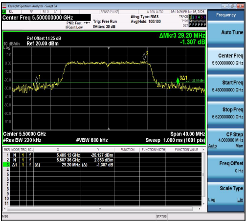
11AC20SISO-Ant1-5500
