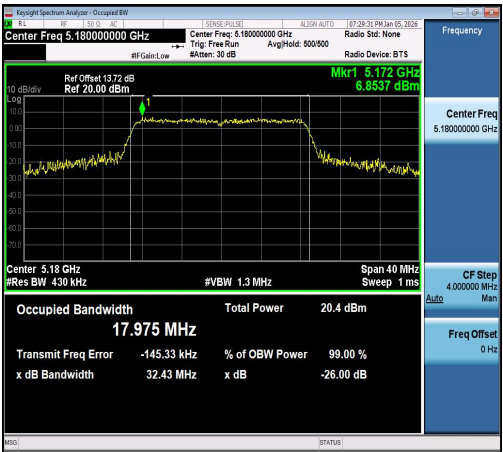
11AC20SISO-Ant1-5180
