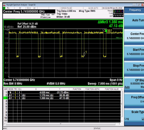
NTNV-11N20SISO-Ant1-5745
