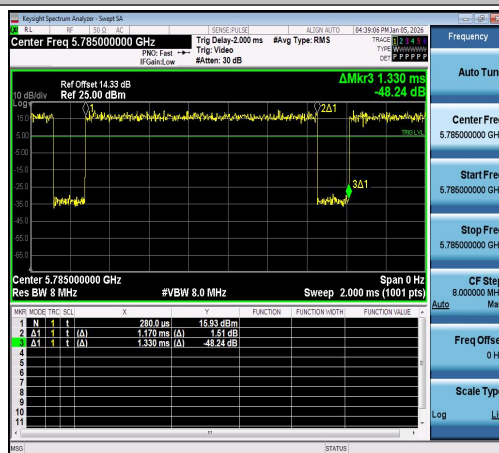
NTNV-11N20SISO-Ant1-5785
