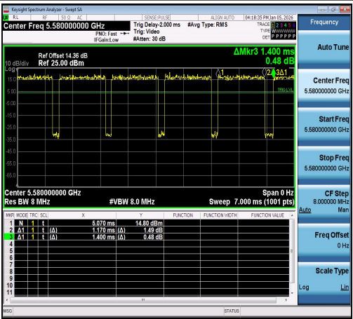
NTNV-11N20SISO-Ant1-5580
