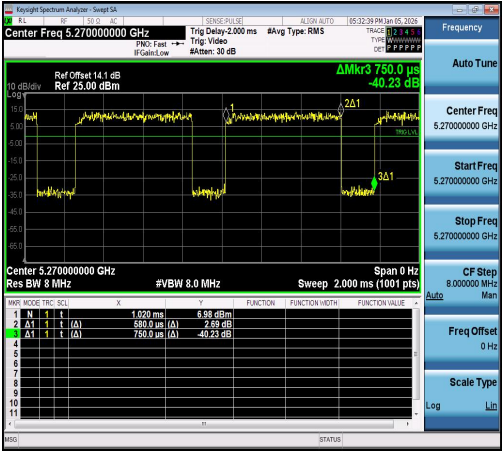
NTNV-11N40SISO-Ant1-5270
