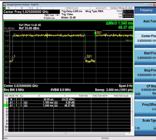
NTNV-11N20SISO-Ant1-5825
