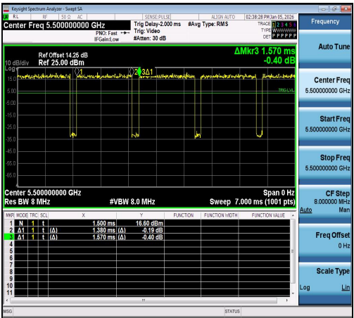
NTNV-11A-Ant1-5500
