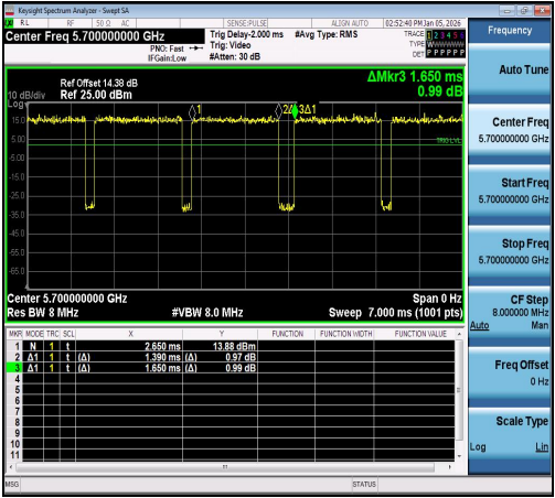
NTNV-11A-Ant1-5700
