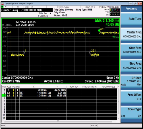
NTNV-11N20SISO-Ant1-5700
