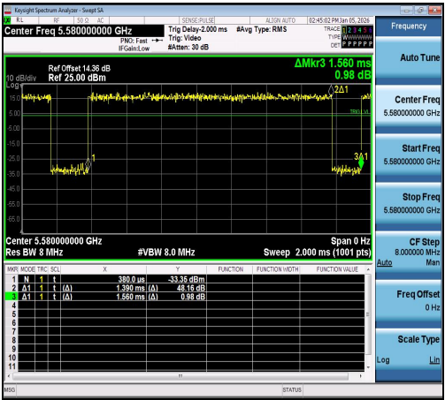
NTNV-11A-Ant1-5580
