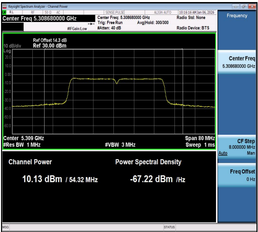
11AC40SISO-Ant1-5310-PASS
