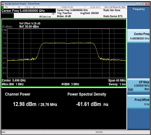
11N20SISO-Ant1-5500-PASS
