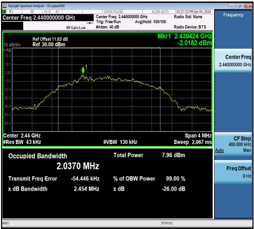
LE_2M-Ant1-2440
