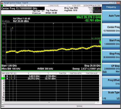
LE_2M-Ant1-2402-1000~26500-PASS
