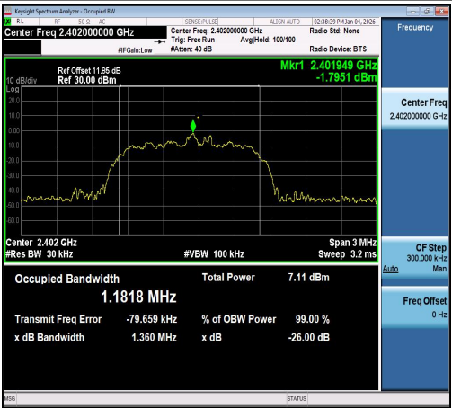
2DH5-Ant1-2402
