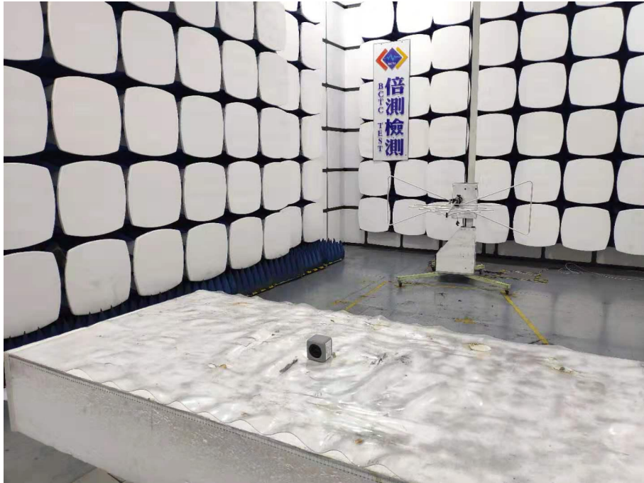
Spurious emissions
