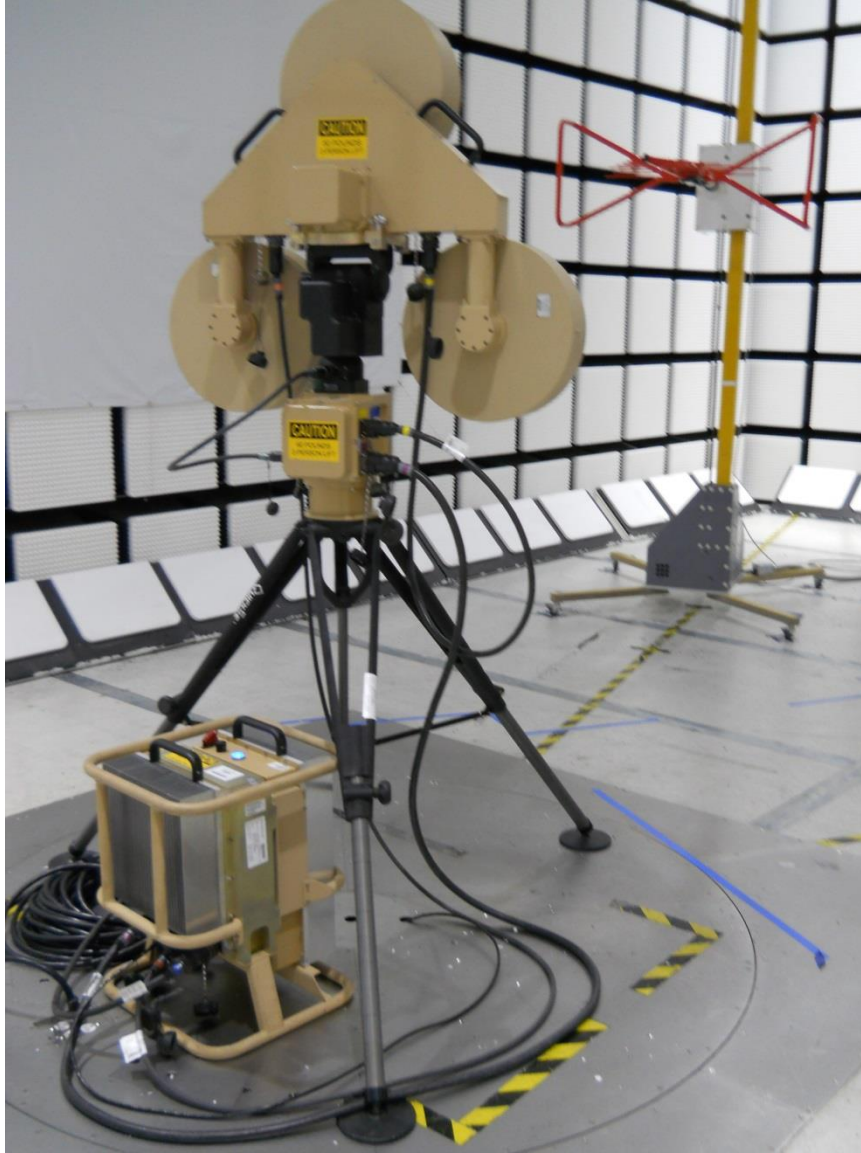
RADIATED EMISSIONS 50-1000 MHz SETUP PHOTO
