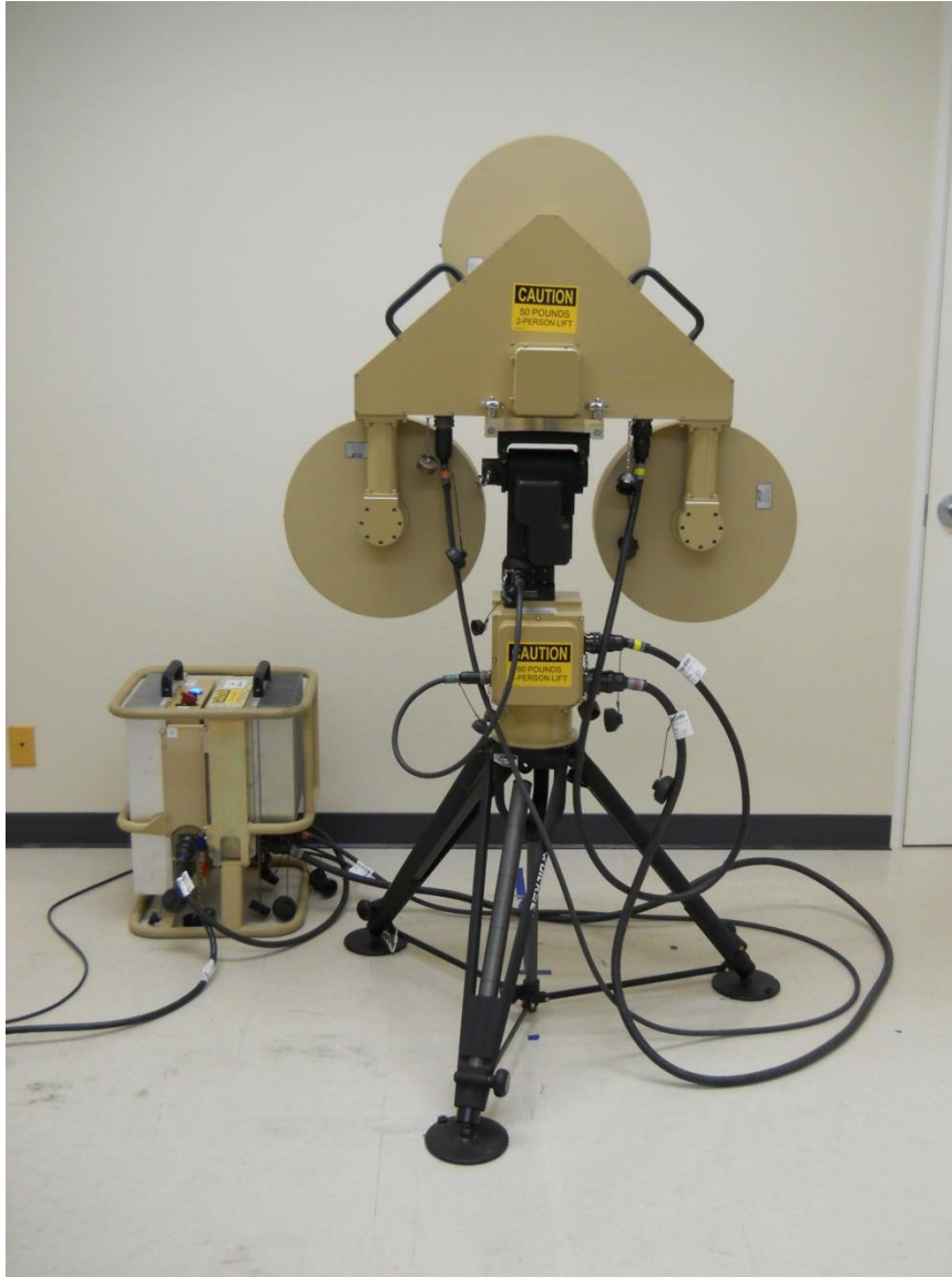
RADIATED EMISSIONS 40-180 GHz SETUP PHOTO - BACK
