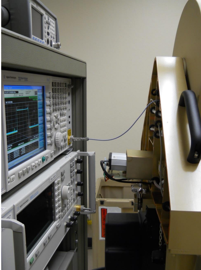
CONDUCTED SETUP PHOTO
