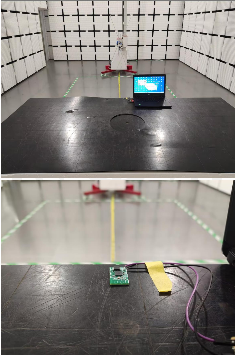
Spurious Radiation Emissions Test (<1G)
