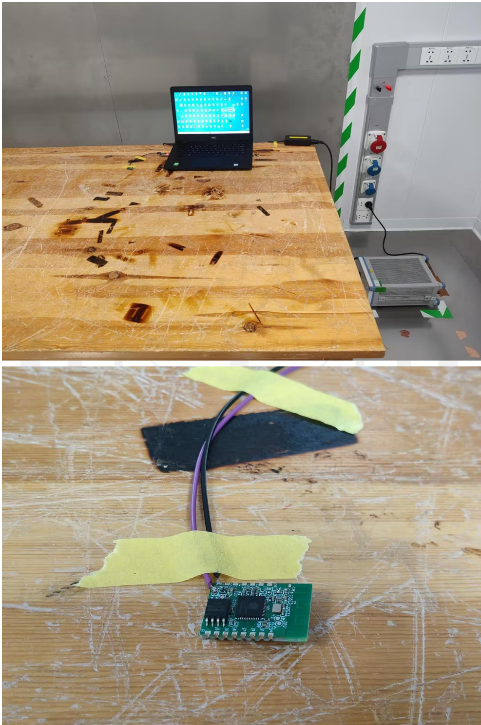
Conducted emission Test
