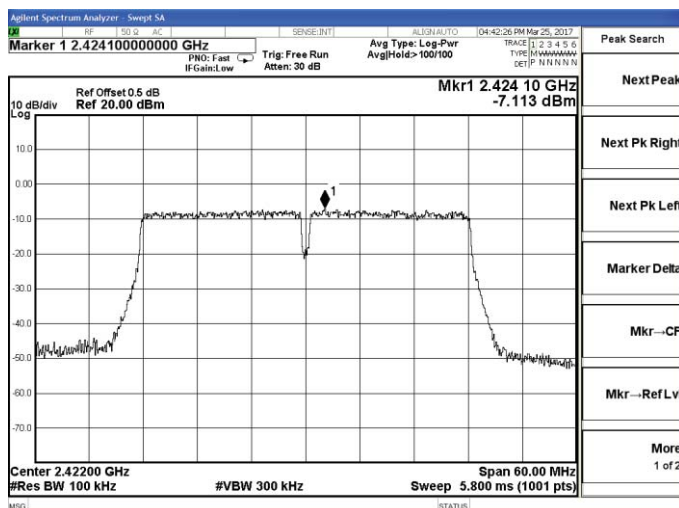
802.11n-HT40-Low channel Reference
