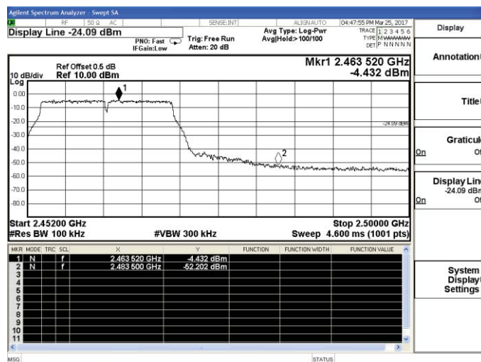
802.11g-High channel
