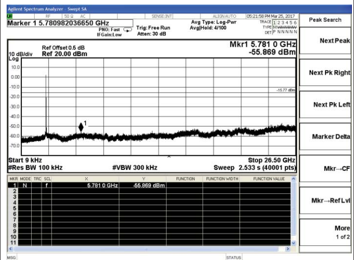
802.11b-Low channel
