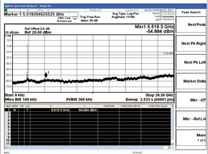
802.11b-High channel
