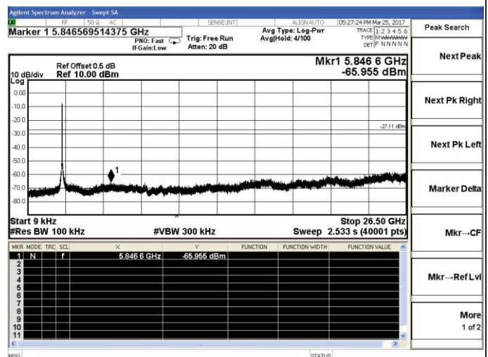
802.11n-HT40-Low channel
