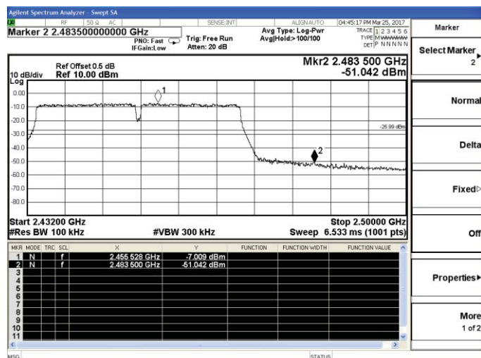
802.11n-HT40-High channel
