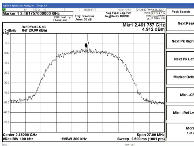
802.11b-High channel Reference
