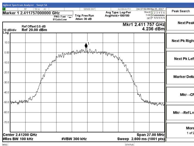
802.11b-Low channel Reference
