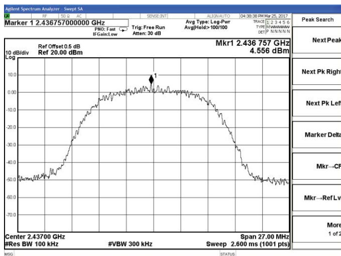
802.11b-Middle channel Reference
