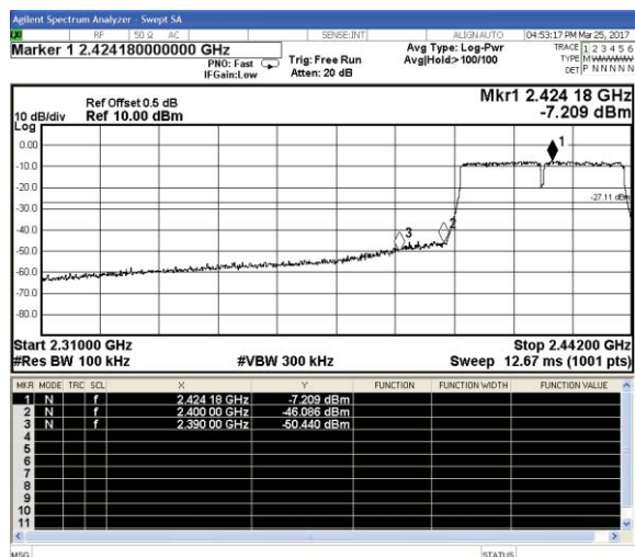
802.11n-HT40-Low channel
