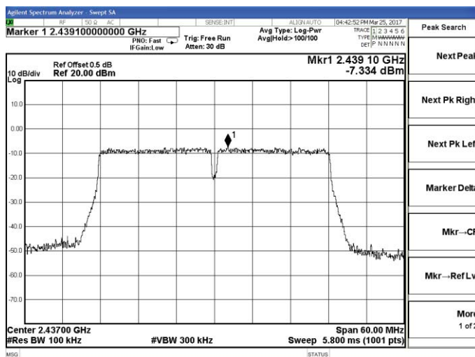
802.11n-HT40-Middle channel Reference
