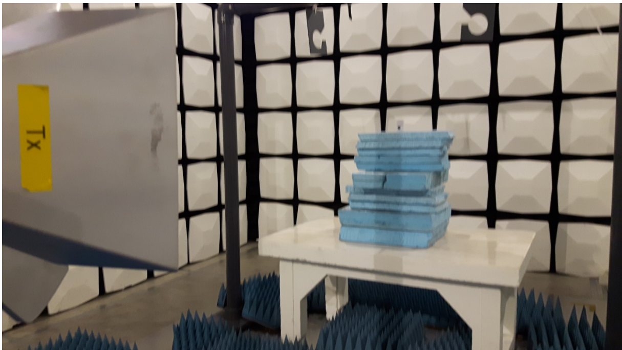
Test set up radiated emission 1GHz – 18 GHz
