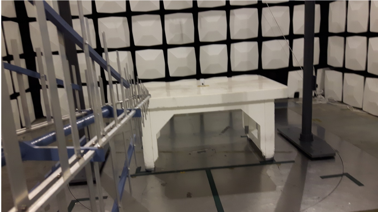
Test set up radiated emission 30 MHz – 1GHz
