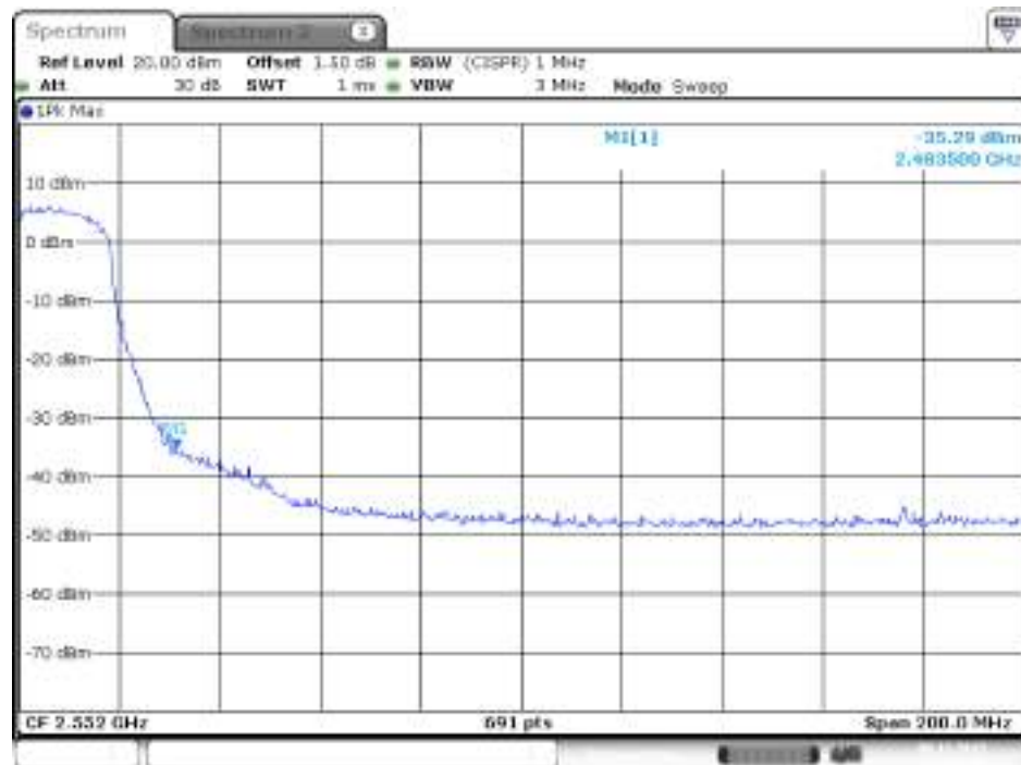
Plot on Configuration IEEE 802.11n MCS0 HT40 / 2452 MHz / Peak / Chain 2
