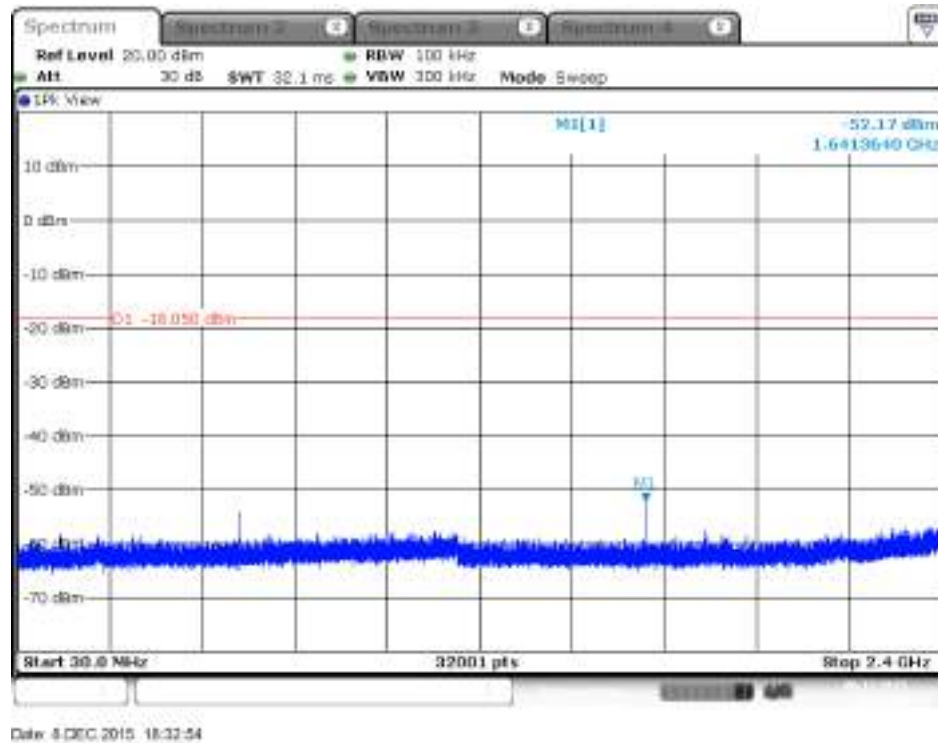
Plot on Configuration IEEE 802.11b / CH 2462 MHz / 30MHz~2400MHz (down 30dBc) / Chain 1
