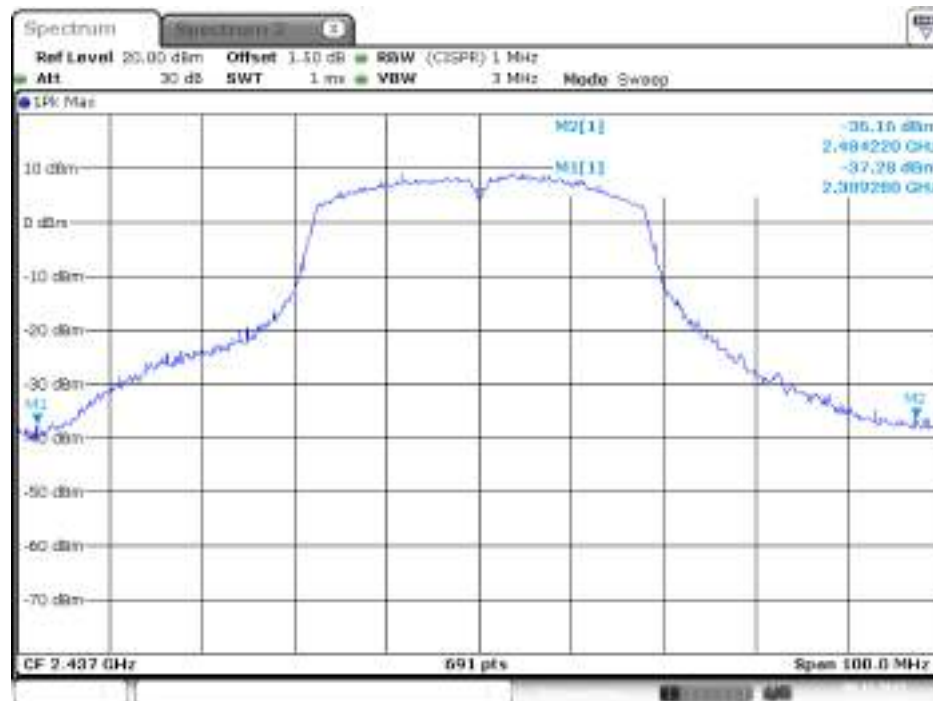
Plot on Configuration IEEE 802.11n MCS0 HT40 / 2437 MHz / Peak / Chain 1
