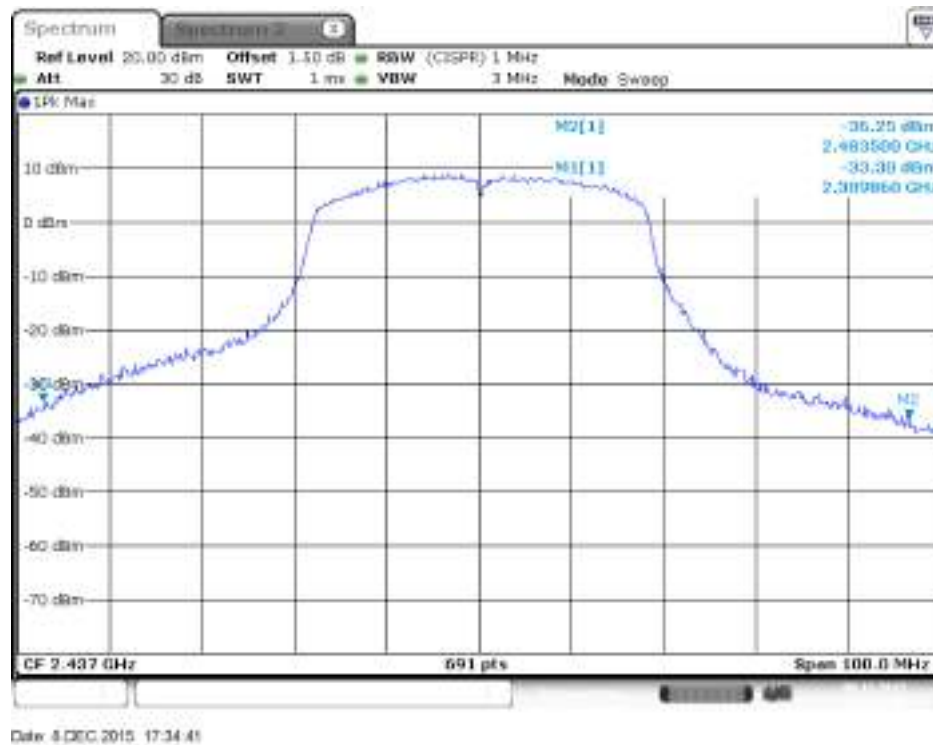
Plot on Configuration IEEE 802.11n MCS0 HT40 / 2437 MHz / Peak / Chain 2
