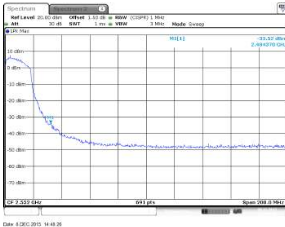
Plot on Configuration IEEE 802.11n MCS0 HT40 / 2452 MHz / Peak / Chain 1
