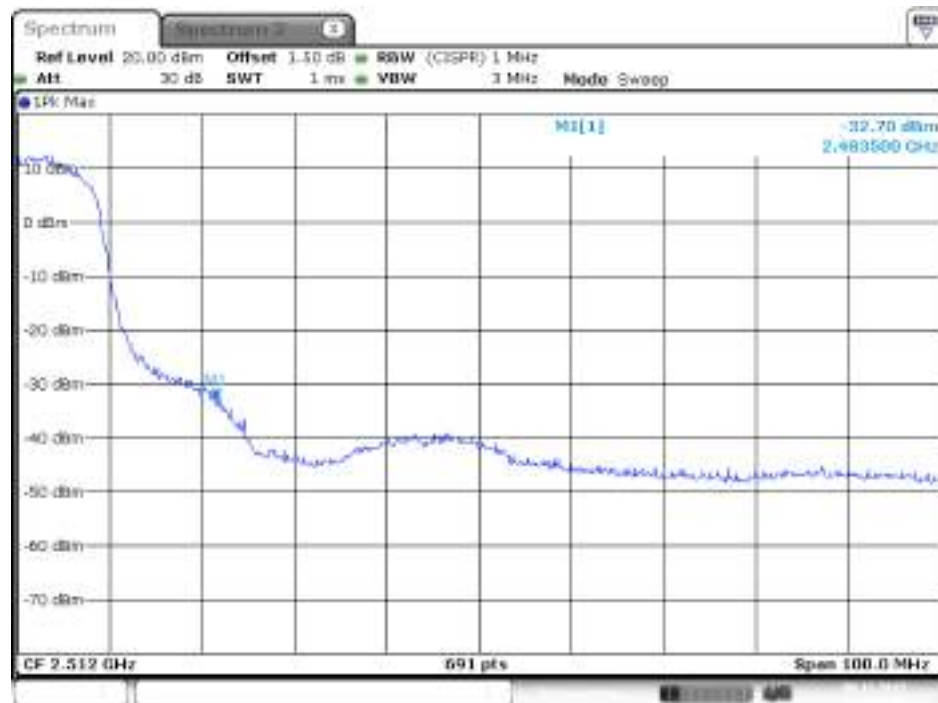
Plot on Configuration IEEE 802.11n MCS0 HT20 / 2462 MHz / Peak / Chain 1
