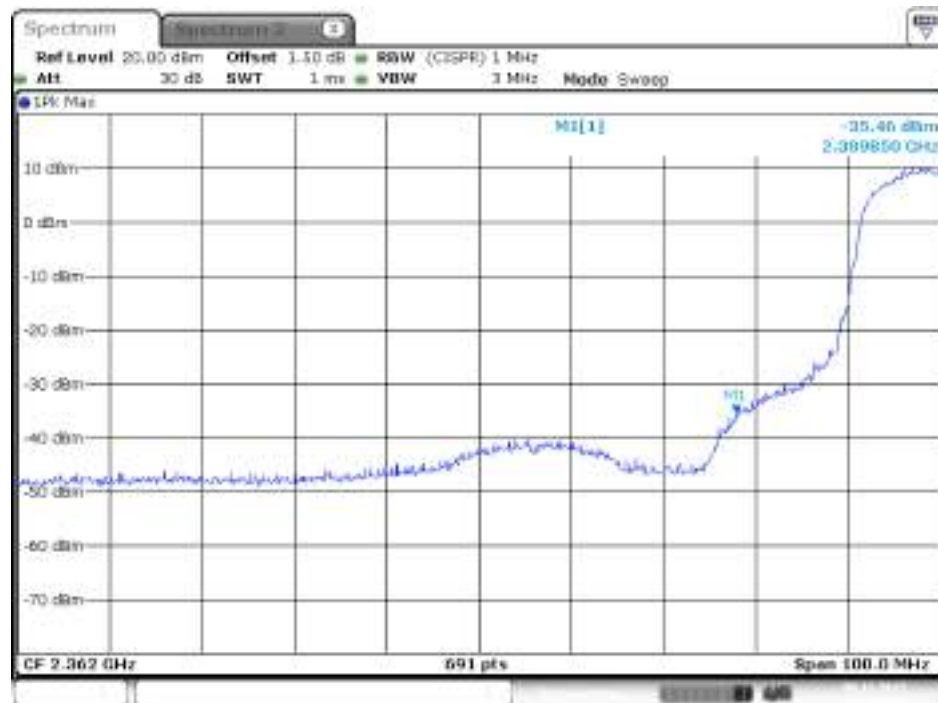
Plot on Configuration IEEE 802.11n MCS0 HT20 / 2412 MHz / Peak / Chain 1
