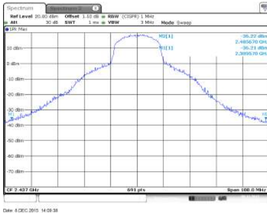
Plot on Configuration IEEE 802.11n MCS0 HT20 / 2437 MHz / Peak / Chain 1
