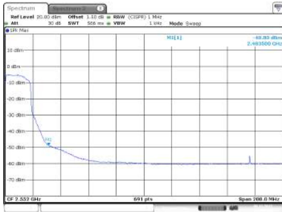
Plot on Configuration IEEE 802.11n MCS0 HT40 / 2452 MHz / Average / Chain 2
