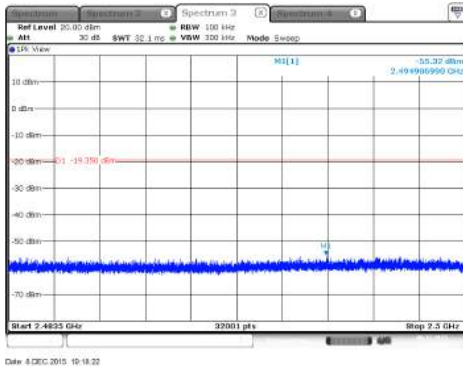
Plot on Configuration IEEE 802.11g / 2412 MHz / 2483.5MHz~2500MHz (down 30dBc) / Chain 1
