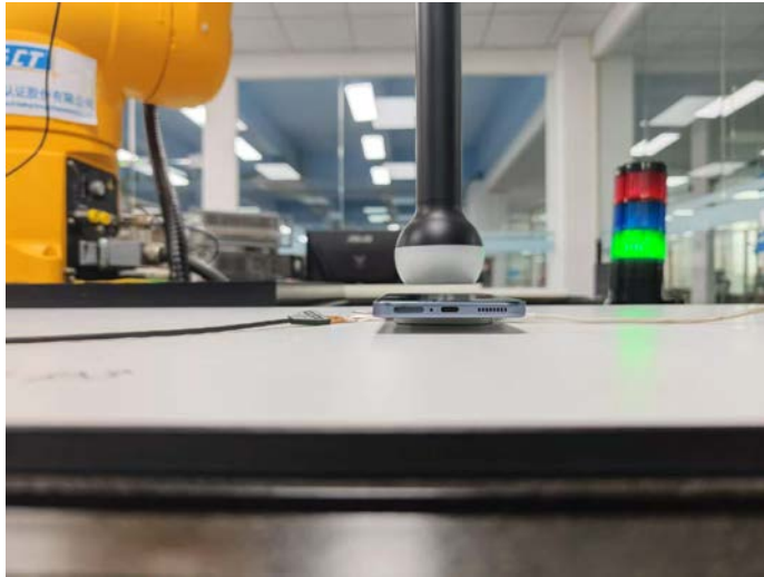
W0300XA WPT Test setup photos
