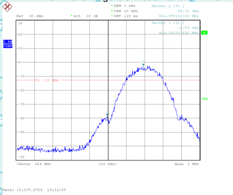
Low Band Edge GSM 850 Band CH 128
