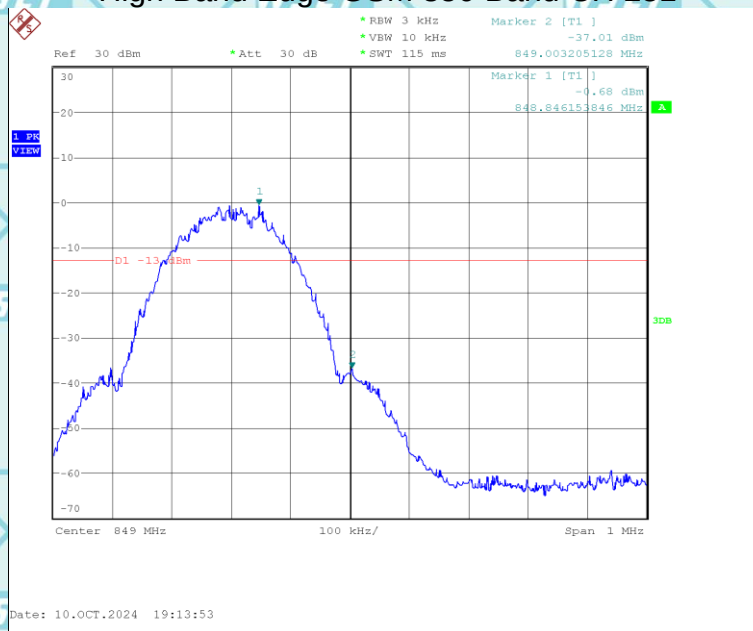
High Band Edge GSM 850 Band CH 251
