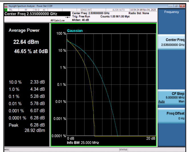
Band7-20MHz-64QAM-21100-100RB#0
