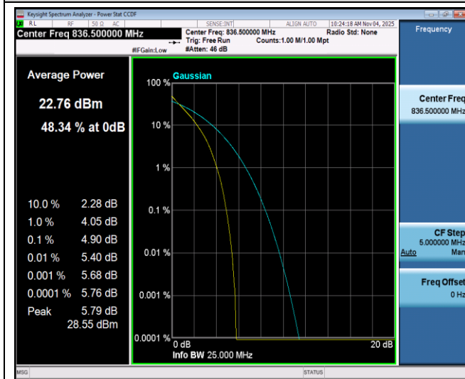
Band5-10MHz-64QAM-20525-50RB#0
