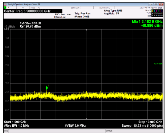
Band5-1.4MHz-64QAM-20643-1RB#0-Range2:1000~10000MHz
