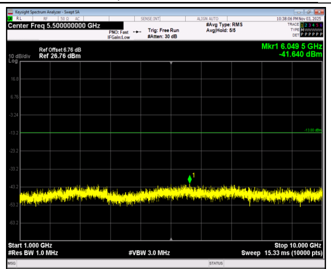
Band5-1.4MHz-16QAM-20407-1RB#0-Range2:1000~10000MHz
