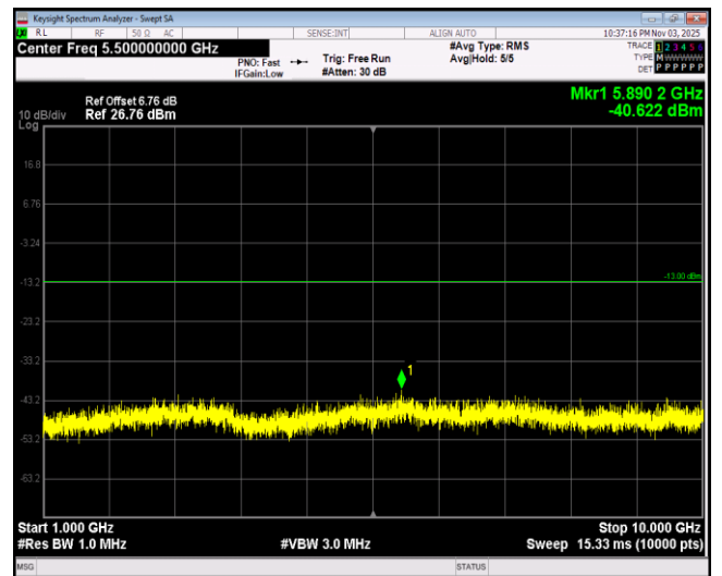
Band5-1.4MHz-QPSK-20643-1RB#0-Range2:1000~1 0000MHz
