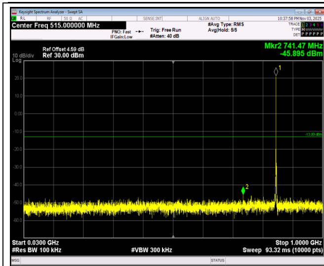
Band5-1.4MHz-16QAM-20407-1RB#0-Range1:30~1000MHz
