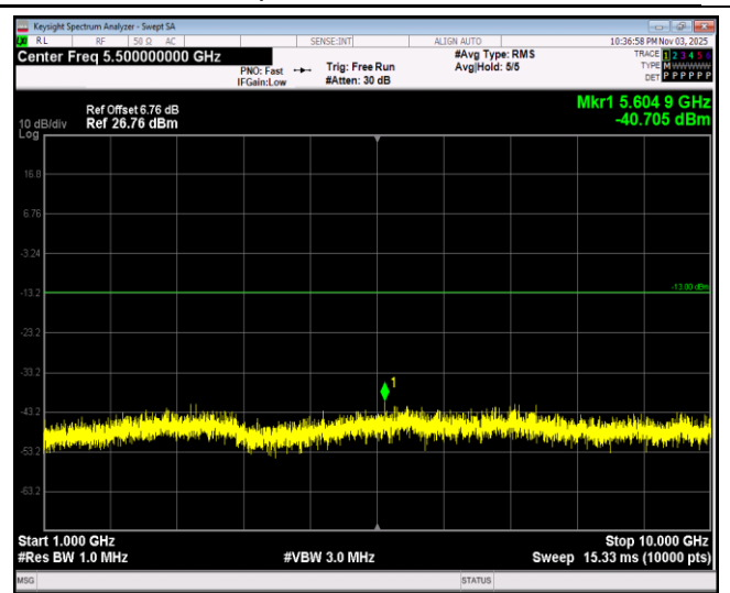
Band5-1.4MHz-64QAM-20525-1RB#0-Range2:1000~10000MHz
