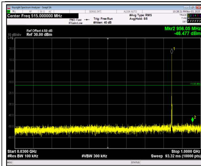
Band5-10MHz-QPSK-20450-1RB#0-Range1:30~100 0MHz
