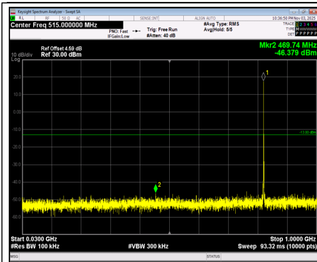
Band5-1.4MHz-64QAM-20525-1RB#0-Range1:30~1000MHz
