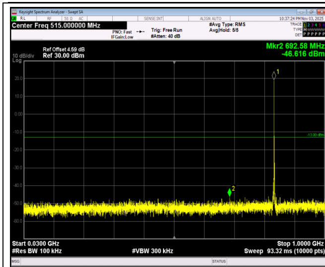
Band5-1.4MHz-16QAM-20643-1RB#0-Range1:30~1000MHz
