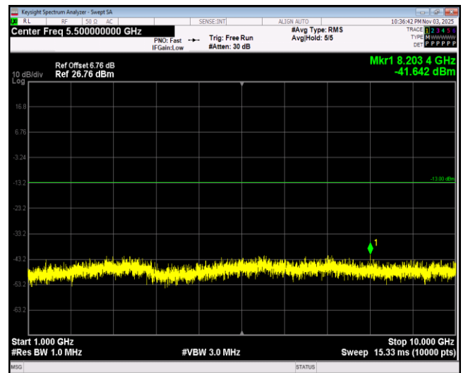
Band5-1.4MHz-16QAM-20525-1RB#0-Range2:1000~10000MHz
