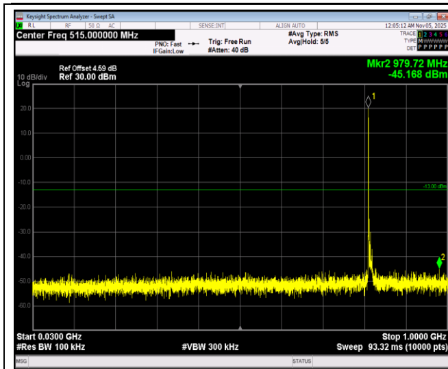
Band26-15MHz-QPSK-26865-1RB#0-Range1:30~1000MHz
