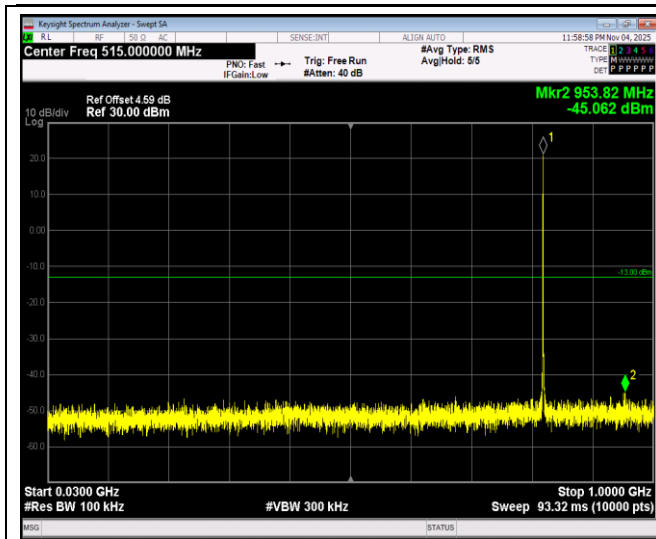
Band26-1.4MHz-64QAM-26797-1RB#0-Range1:30~1000MHz
