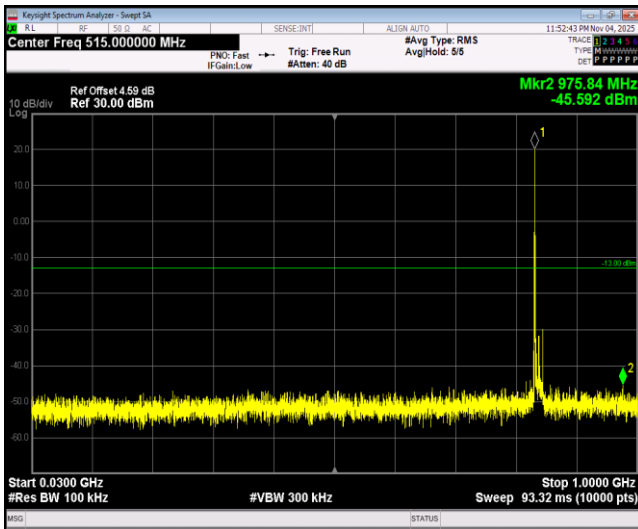
Band38-5MHz-QPSK-37775-1RB#0-Range1:30~1000MHz
