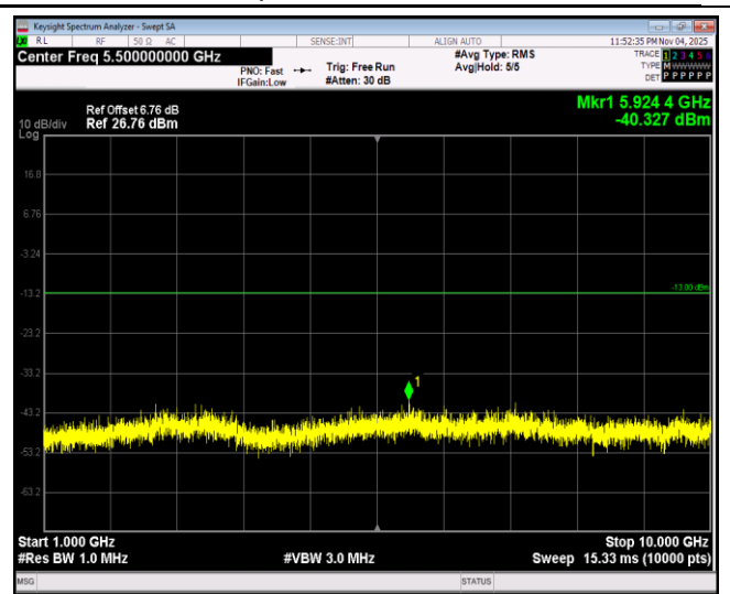
Band26-15MHz-64QAM-26965-1RB#0-Range2:1000~10000MHz
