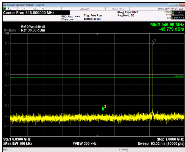
Band26-1.4MHz-64QAM-26915-1RB#0-Range1:30~1000MHz
