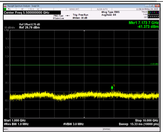
Band26-1.4MHz-64QAM-26740-1RB#0-Range2:1000~10000MHz
