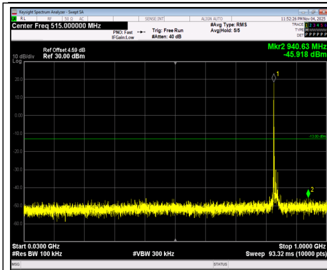
Band26-15MHz-64QAM-26965-1RB#0-Range1:30~1000MHz
