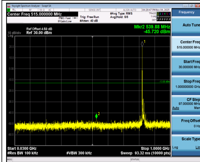
Band26-15MHz-QPSK-26915-1RB#0-Range1:30~1000MHz
