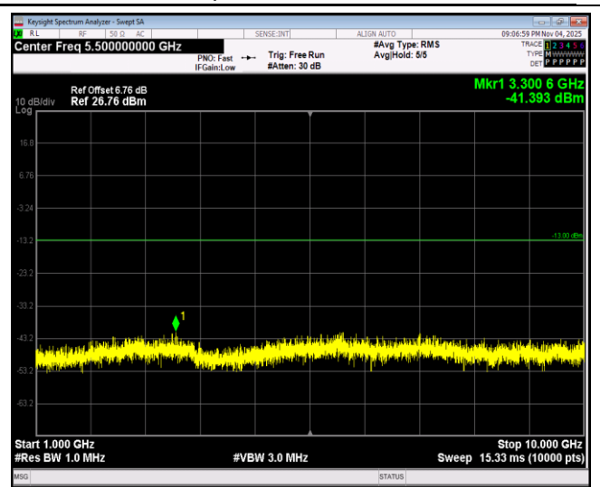
Band26-1.4MHz-64QAM-27033-1RB#0-Range2:1000~10000MHz
