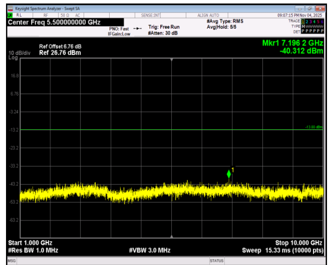
Band26-10MHz-QPSK-26740-1RB#0-Range2:1000~10000MHz
