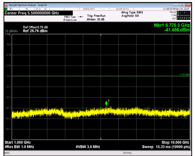
Band26-1.4MHz-64QAM-26783-1RB#0-Range2:1000~10000MHz
