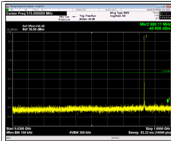
Band26-1.4MHz-64QAM-27033-1RB#0-Range1:30~1000MHz
