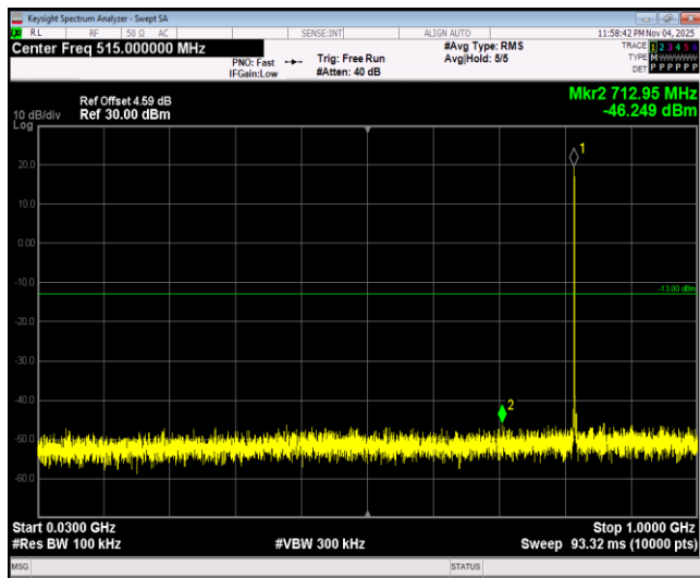
Band26-1.4MHz-64QAM-26783-1RB#0-Range1:30~1000MHz
