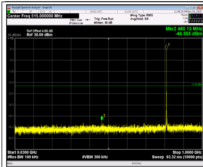
Band26-1.4MHz-64QAM-26740-1RB#0-Range1:30~1000MHz
