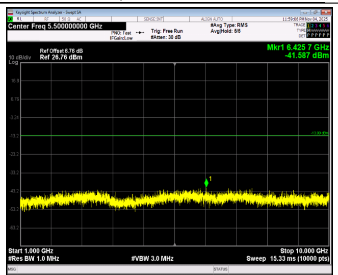
Band26-1.4MHz-64QAM-26797-1RB#0-Range2:1000~10000MHz
