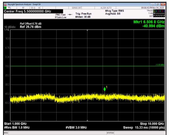
Band26-1.4MHz-64QAM-26915-1RB#0-Range2:1000~10000MHz
