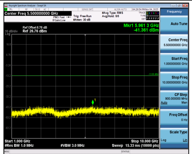
Band26-15MHz-QPSK-26915-1RB#0-Range2:1000~10000MHz
