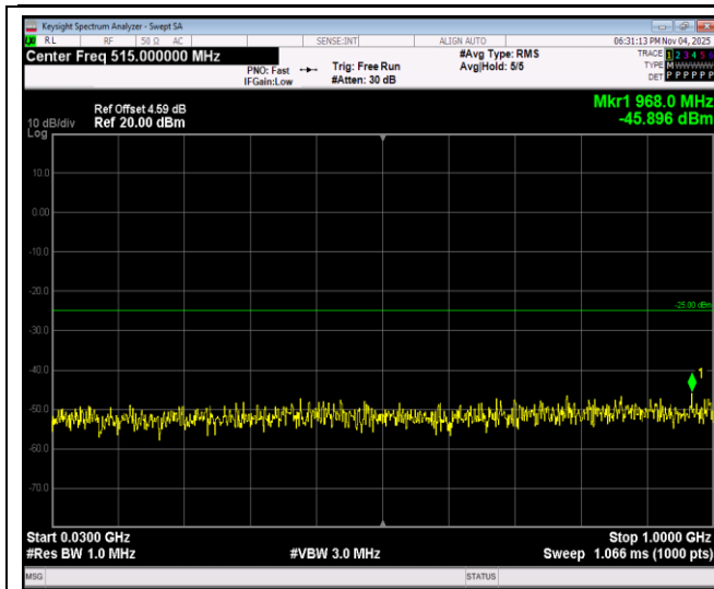
Band41-20MHz-QPSK-41490-1RB#0-Range1:30~1000MHz
