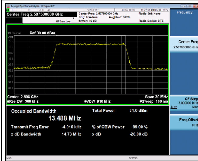
Band7-15MHz-QPSK-21375-75RB#0
