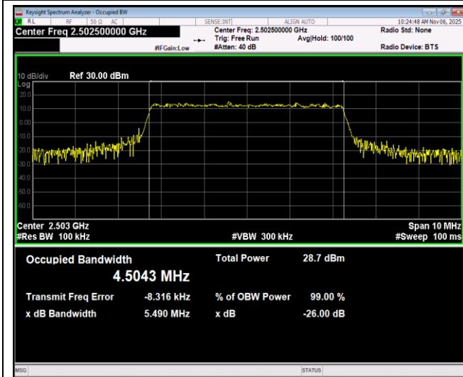
Band7-5MHz-64QAM-21425-25RB#0
